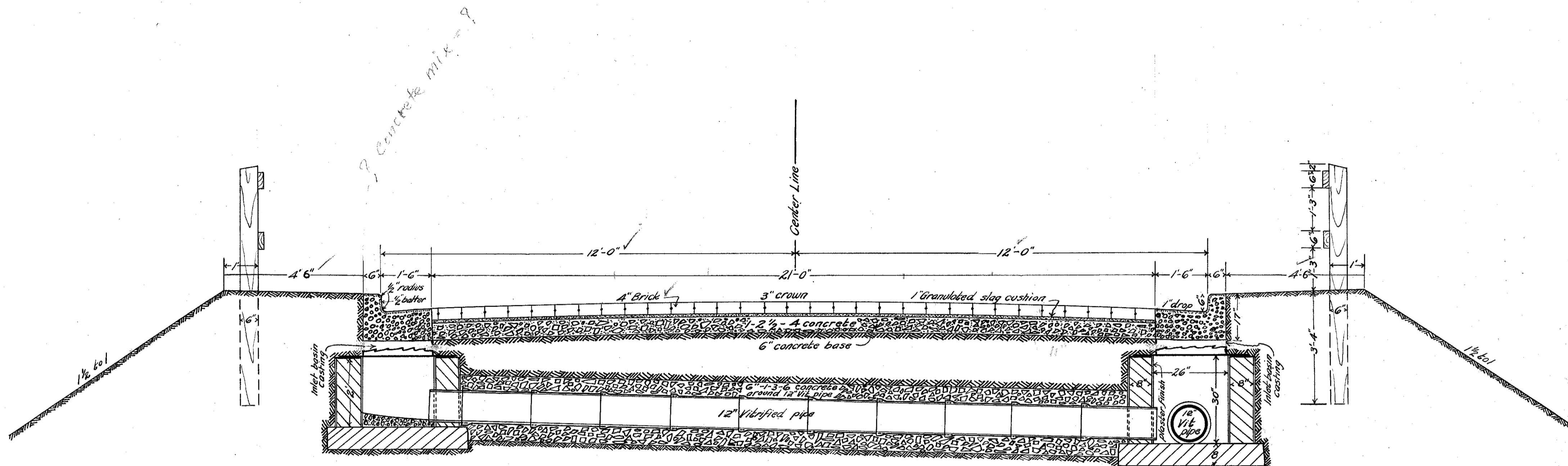
TYPICAL SECTION SCALE 1"=2'
