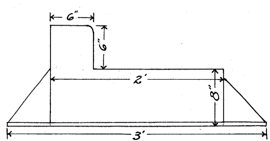
INLET BASIN CASTING
