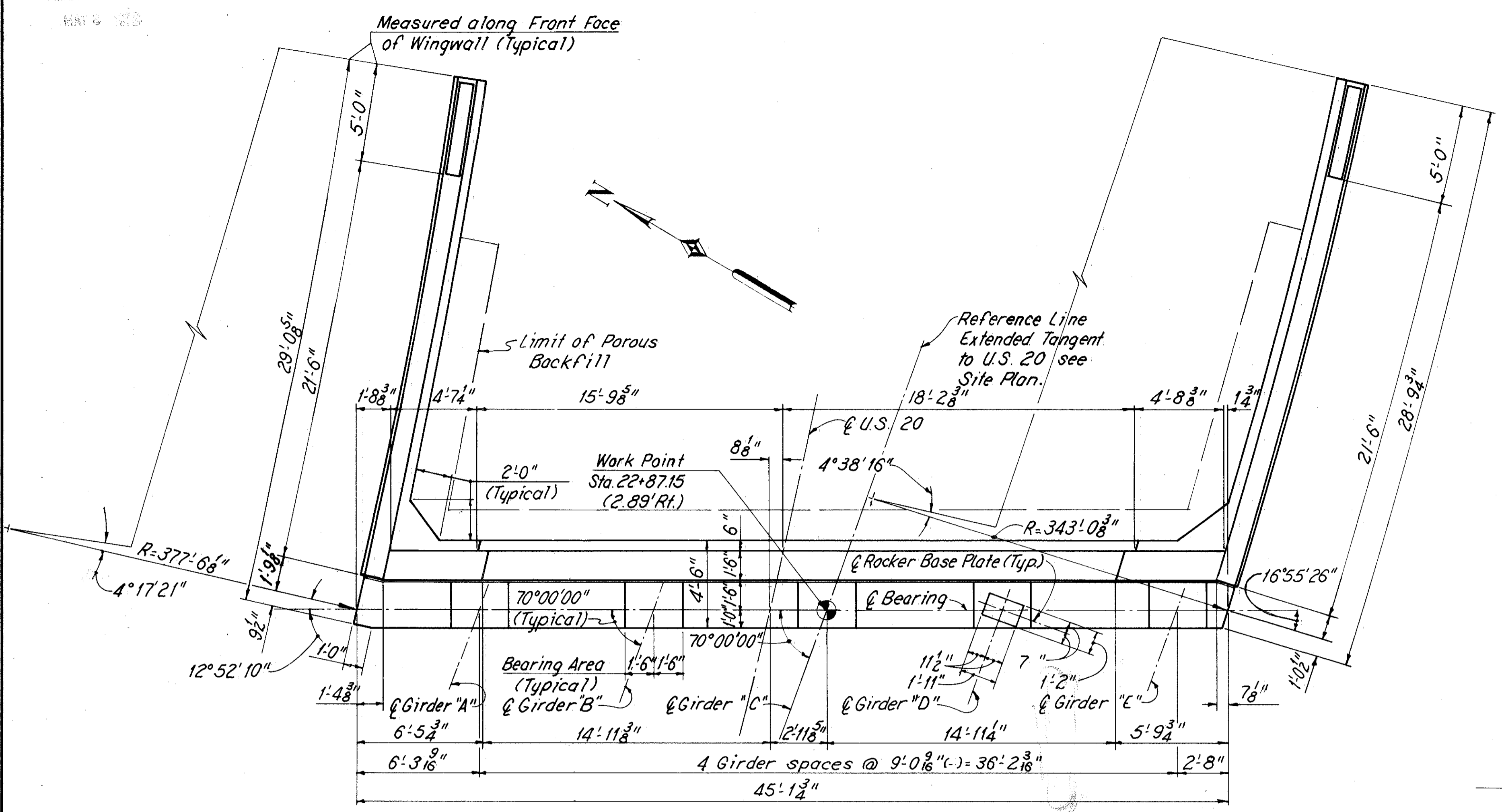
PLAN
