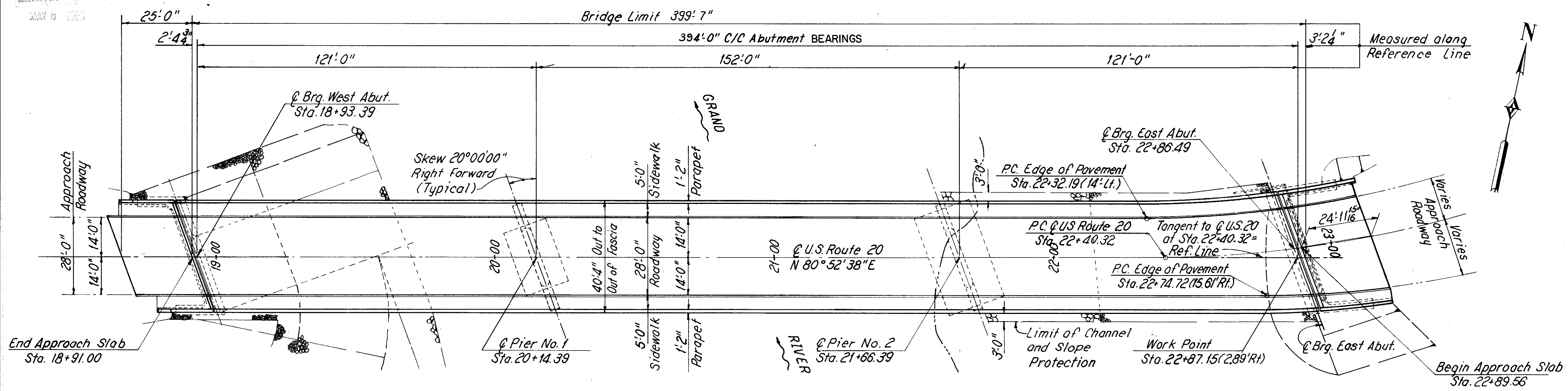
GENERAL PLAN
