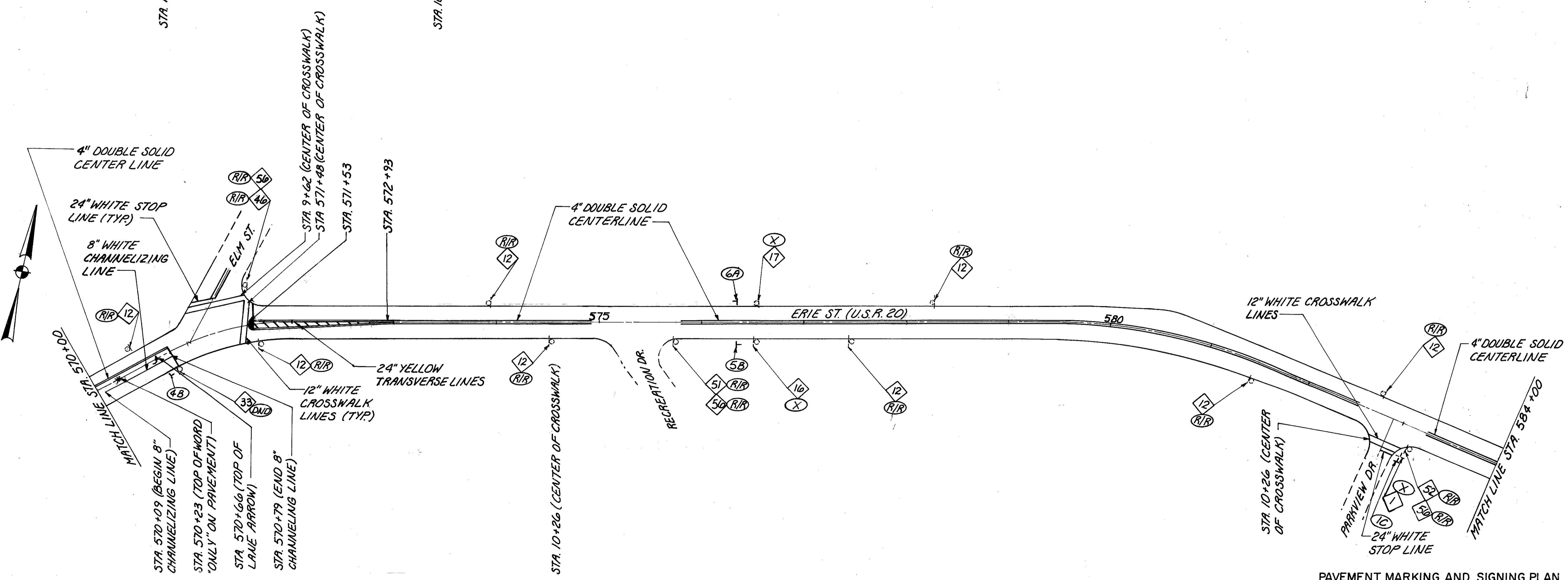
PAVEMENT MARKING AND SIGNING PLAN
