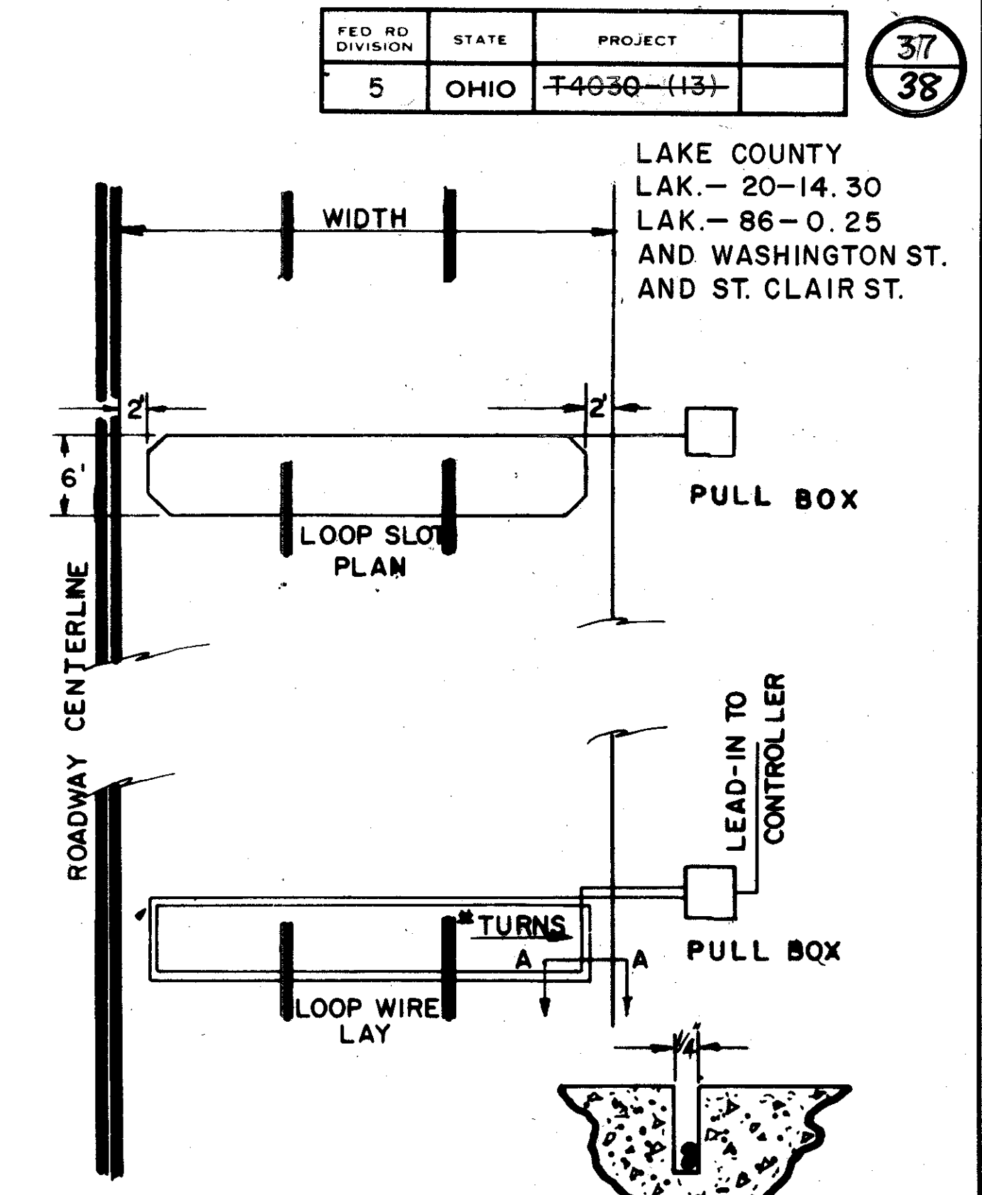
FIGURE 4 TYPICAL THREE LANE LOOP INSTALLATION
