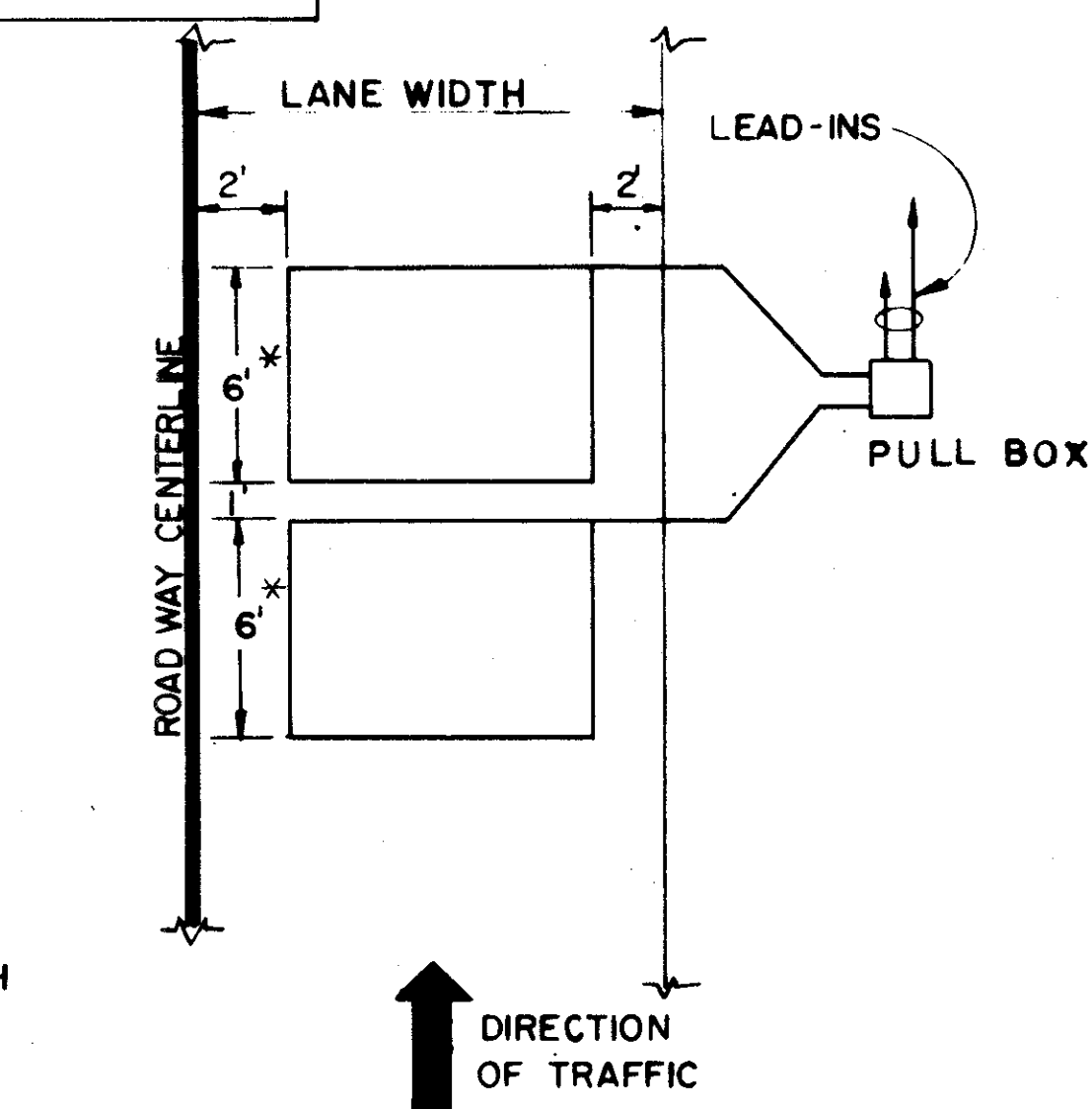
FIGURE 7 TYPICAL DIRECTIONAL DETECTION LOOP INSTALLATION (ADJACENT)
