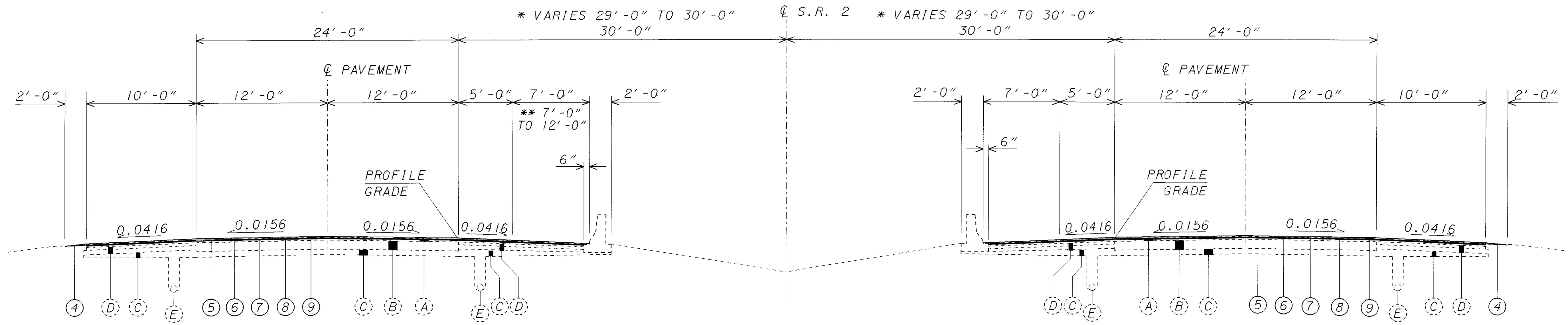
NORMAL SECTION WITH CONCRETE MEDIAN BARRIER, TYPE D
