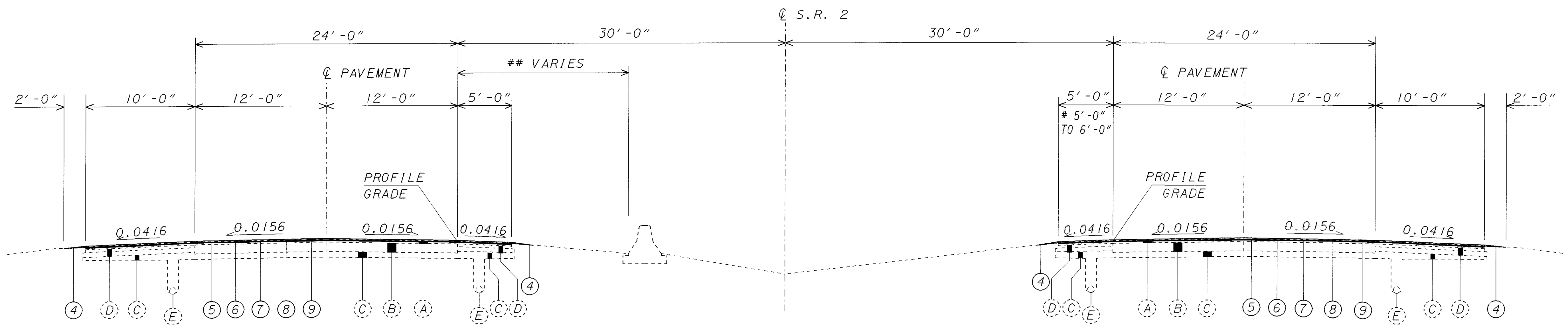
NORMAL SECTION WITH CONCRETE MEDIAN BARRIER, TYPE B
