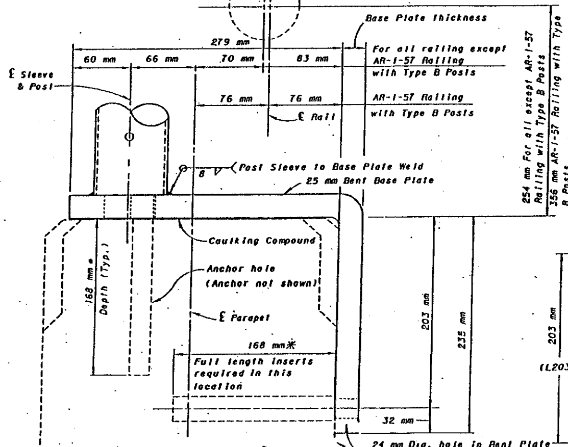
END VIEW BP-3
