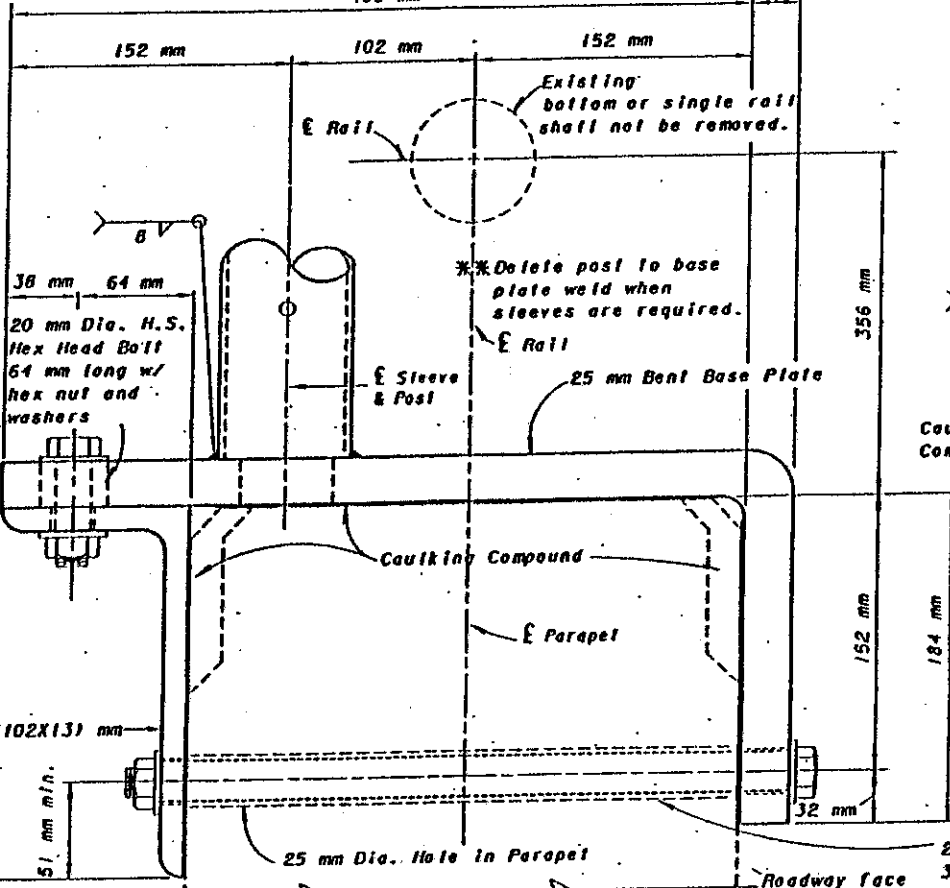
END VIEW BP-4
