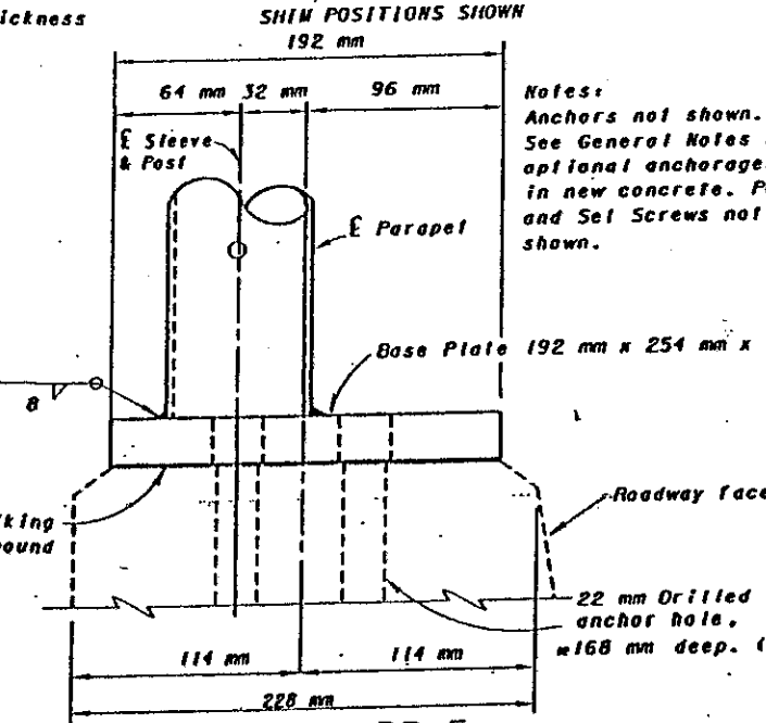
END VIEW BP-5
