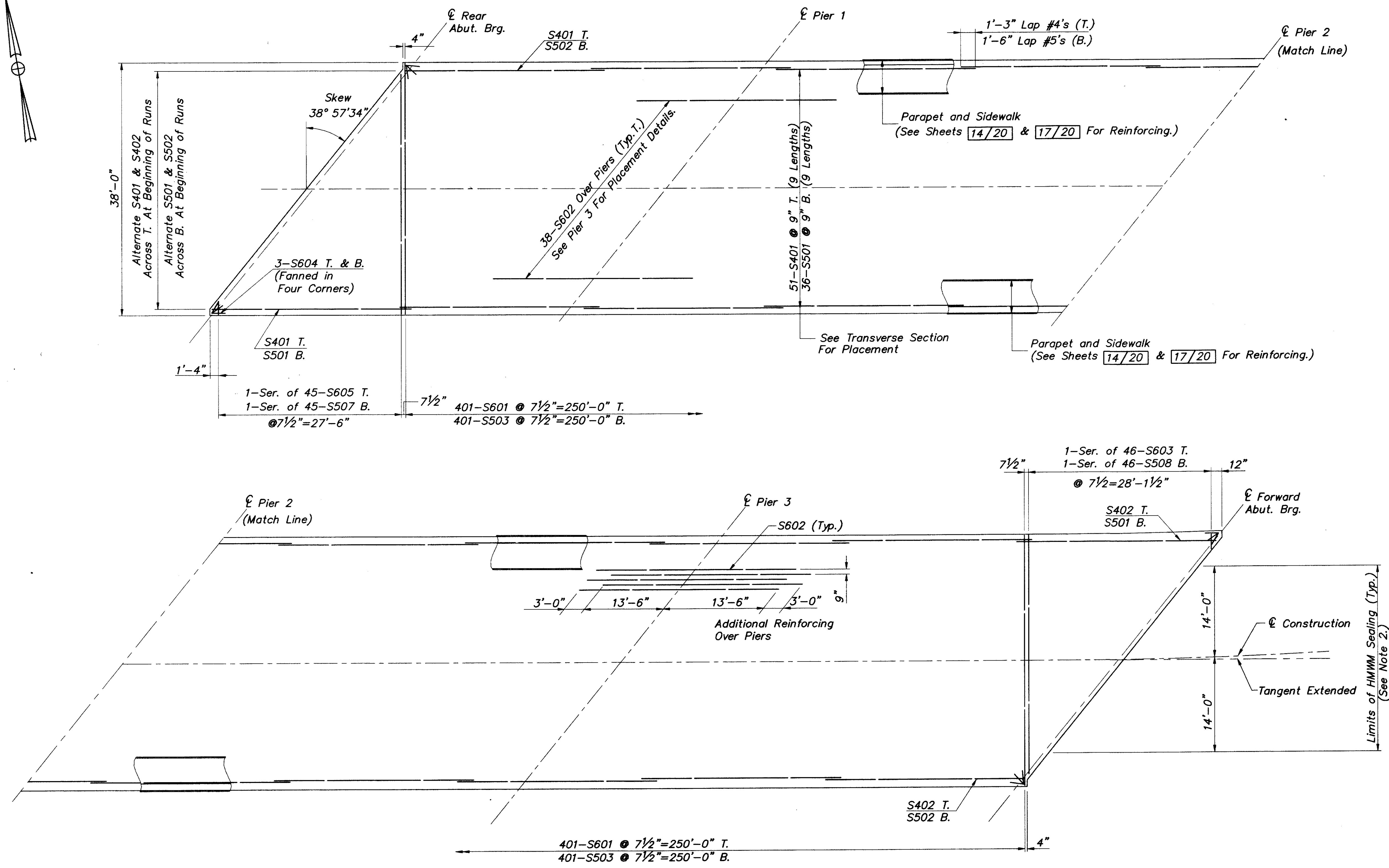
SLAB REINFORCING PLAN
