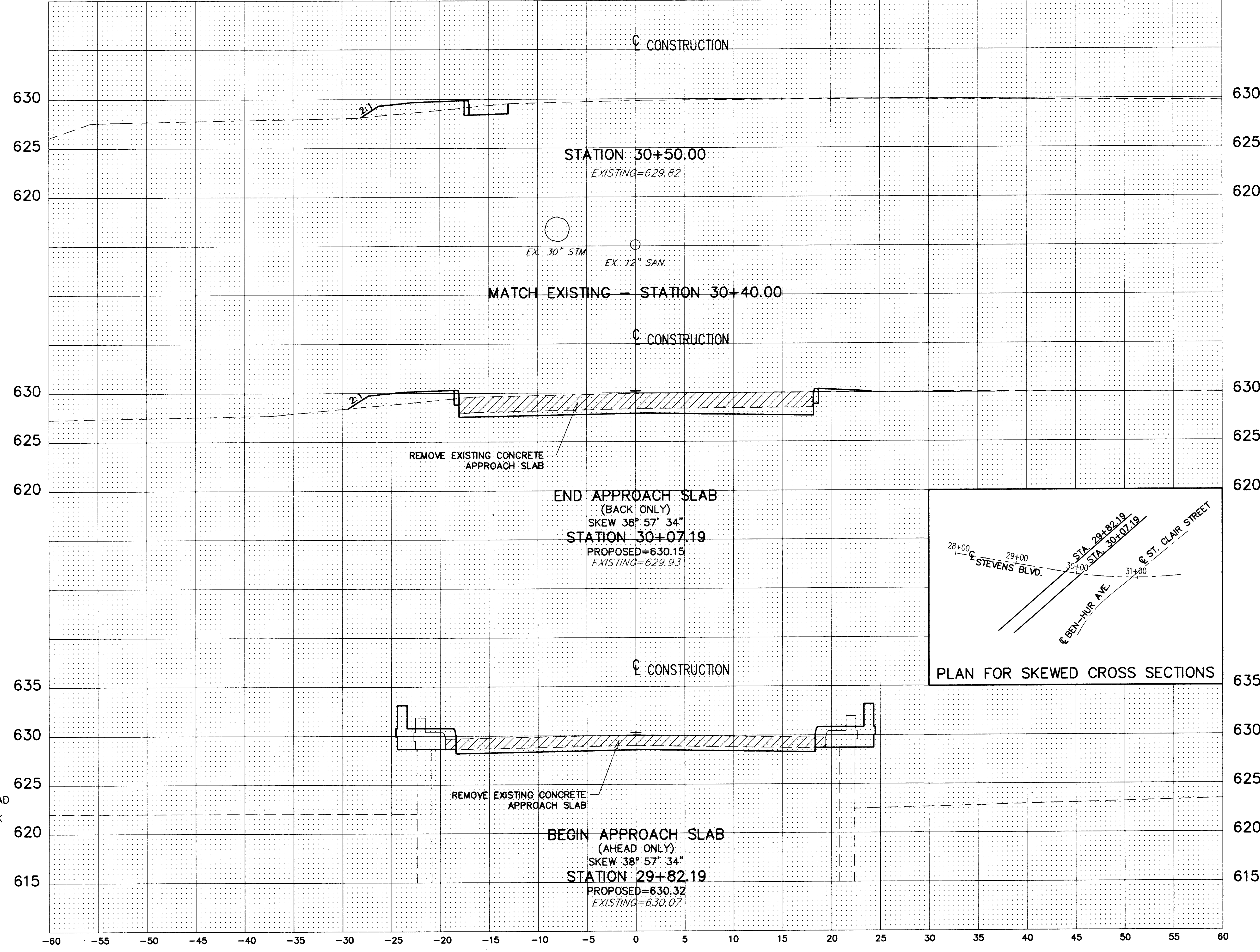
CROSS SECTION STA.29+82.19 TO STA.30+50
