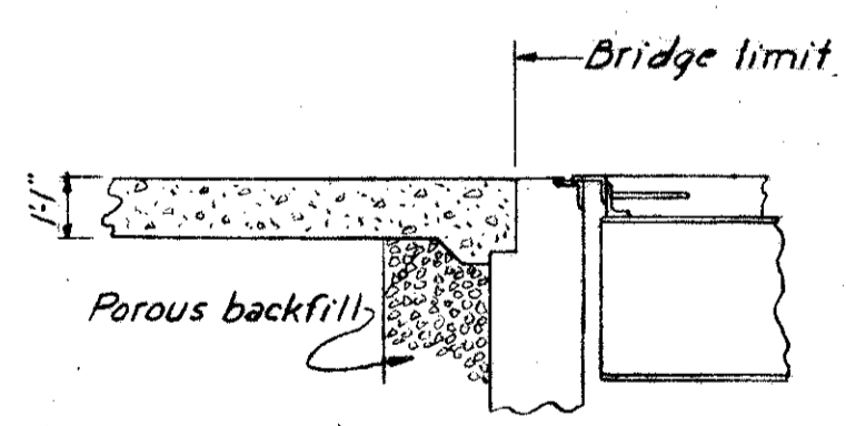
TYPICAL SECTION OF SLAB AT BRIDGE
