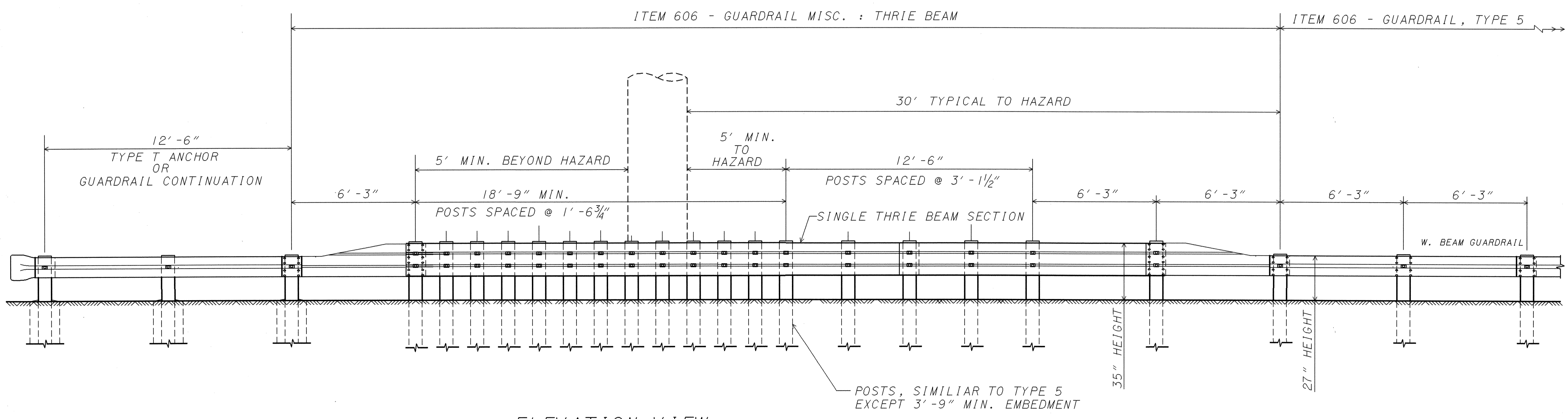
ELEVATION VIEW
