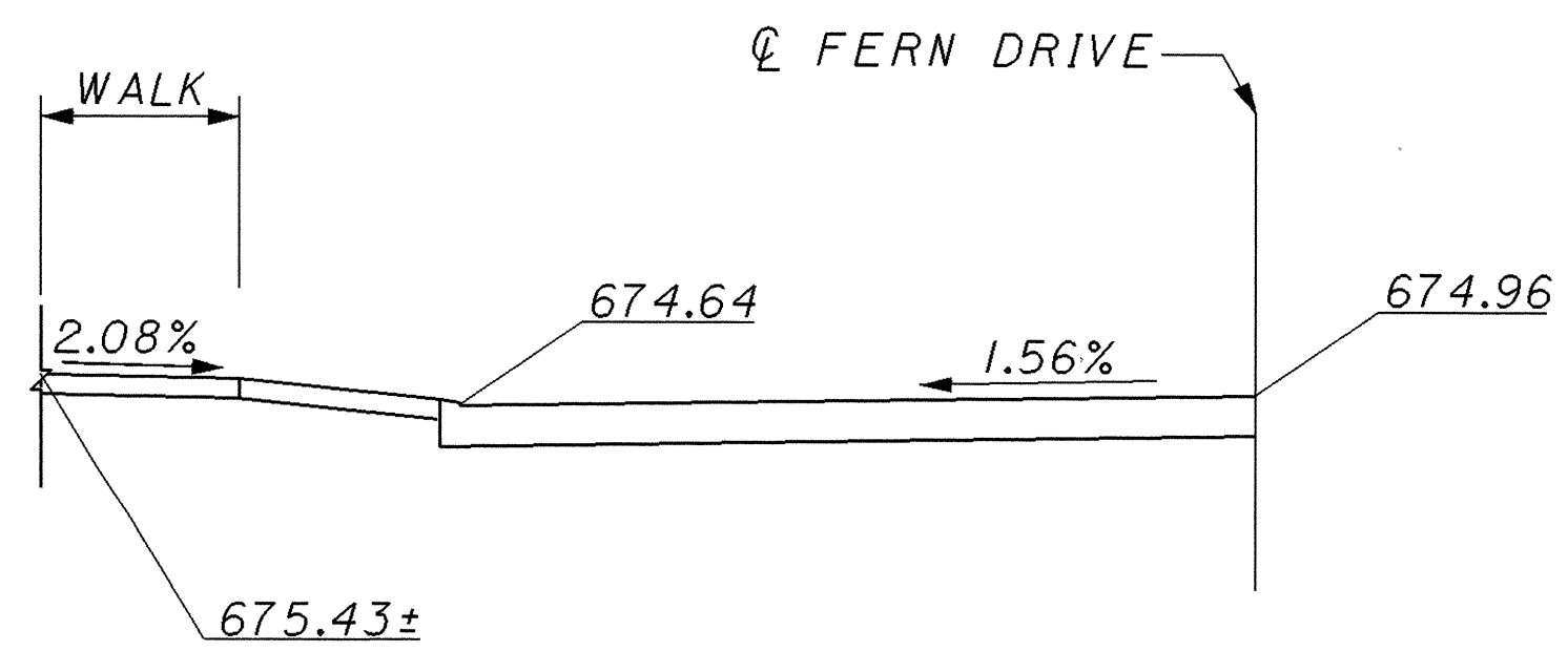
DETAIL B-B
