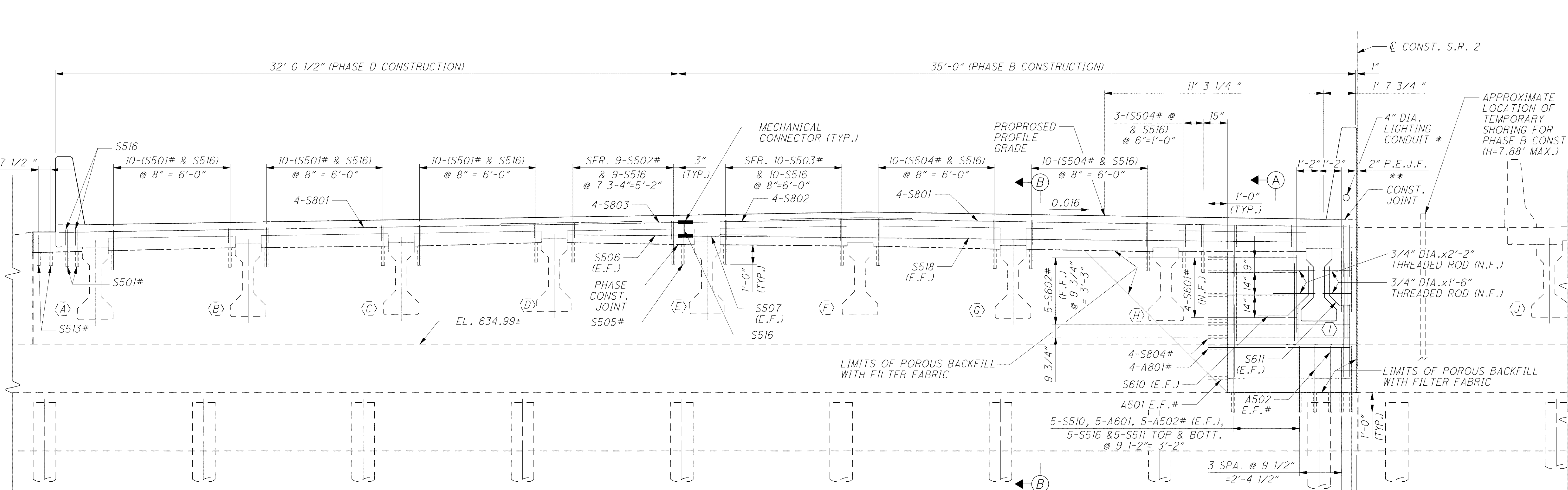
ELEVATION (LEFT FORWARD ABUTMENT SHOWN, LEFT REAR ABUTMENT SIMILAR)
