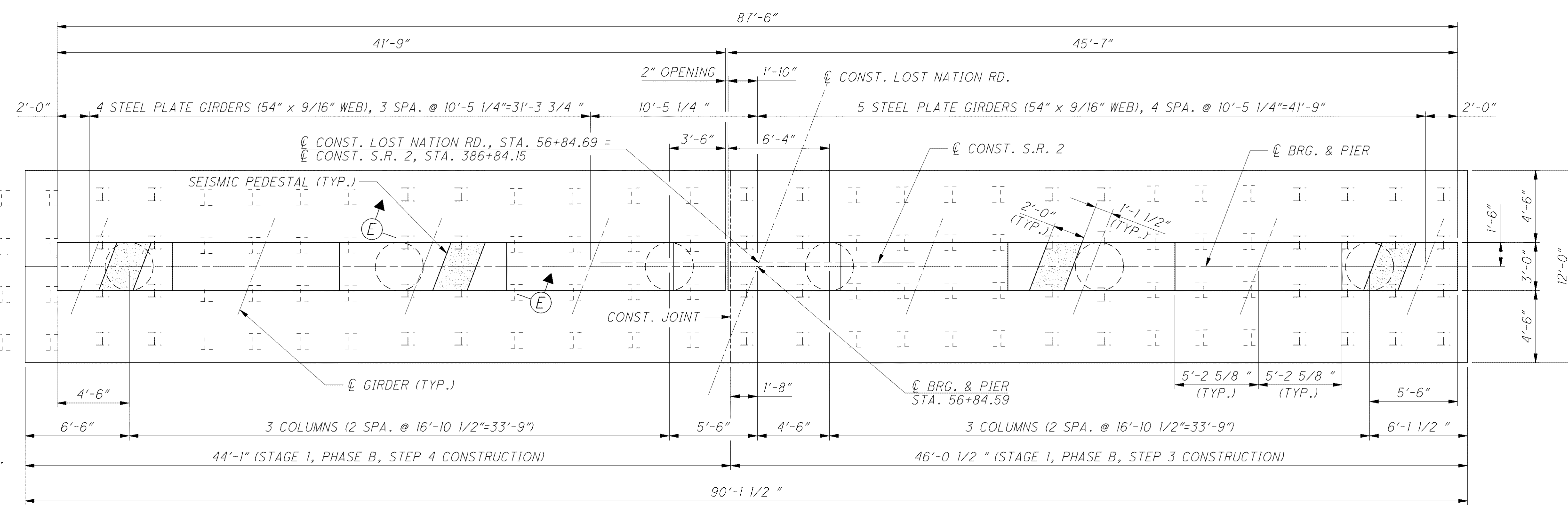
PLAN
