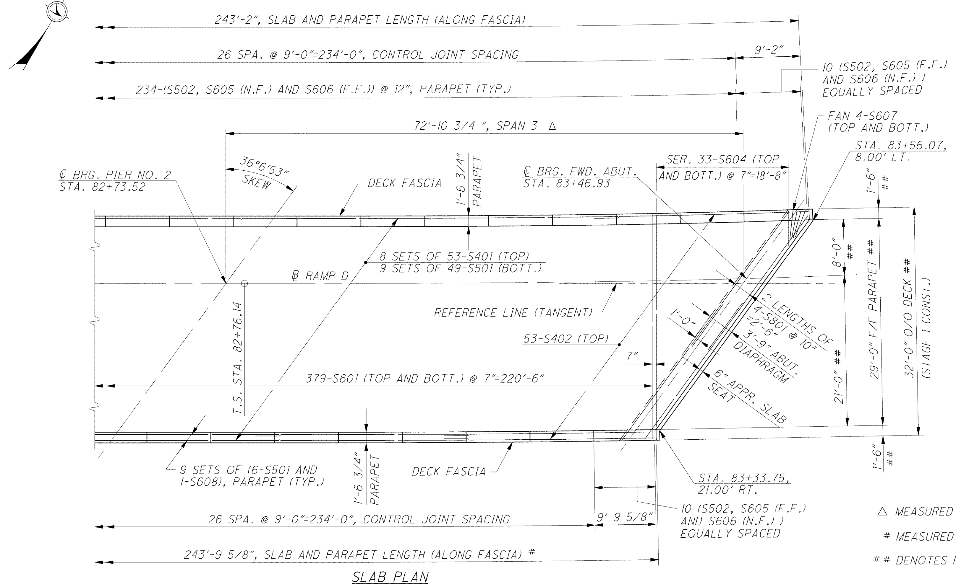
SLAB PLAN
