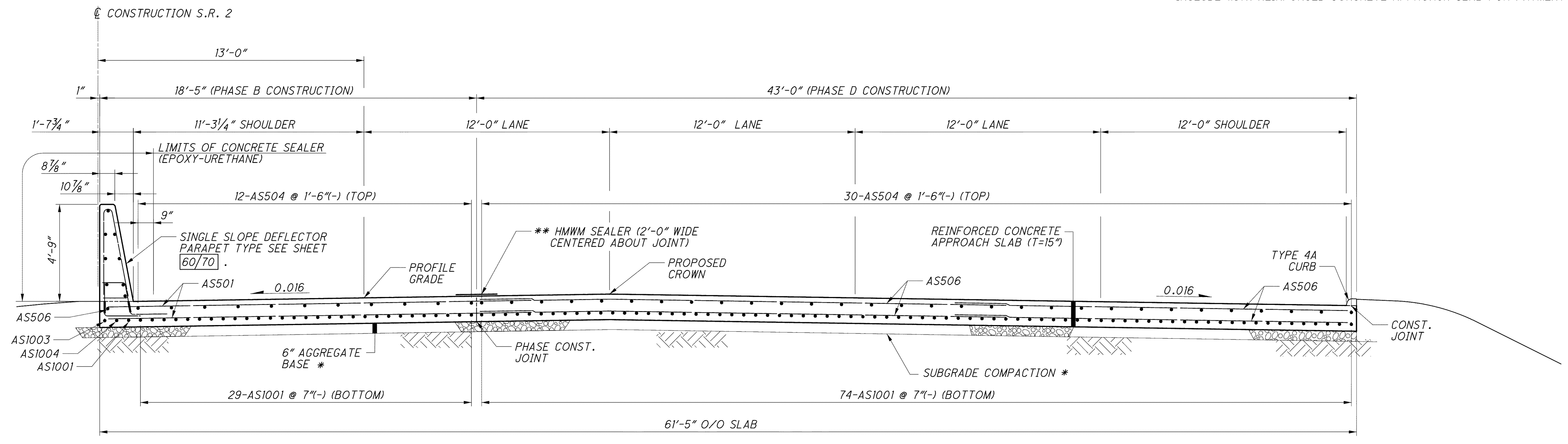
APPROACH SLAB TYPICAL SECTION EASTBOUND FORWARD
