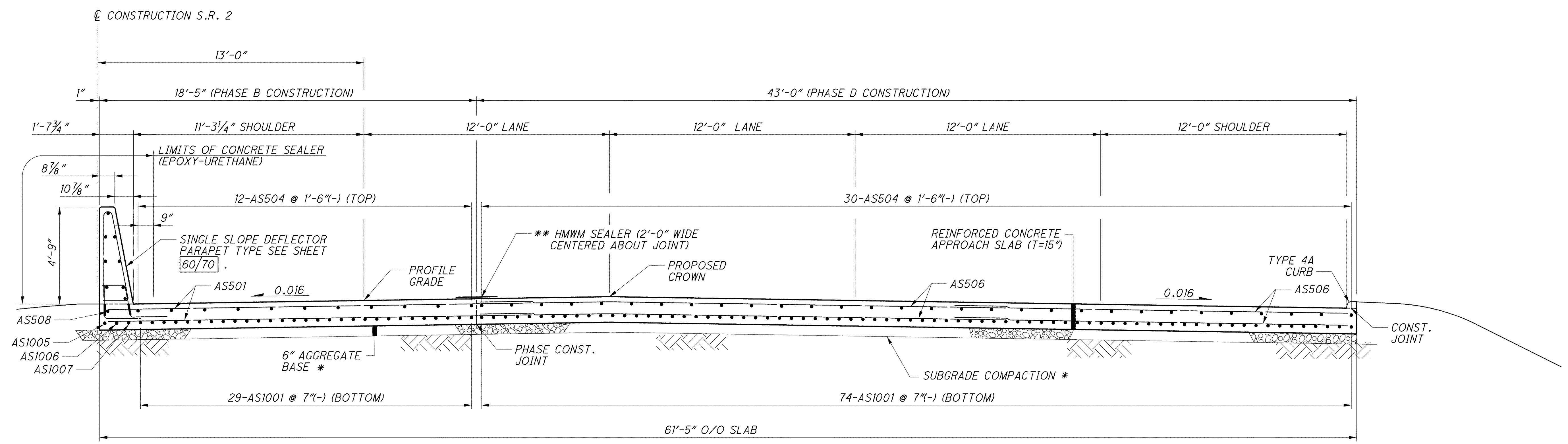
APPROACH SLAB TYPICAL SECTION EASTBOUND REAR
