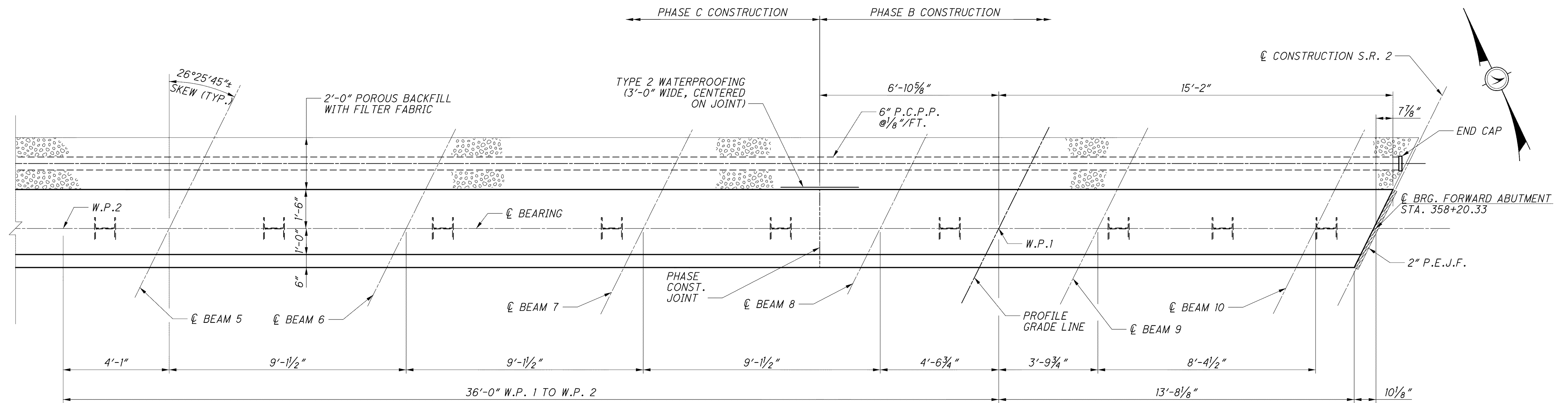
PLAN
