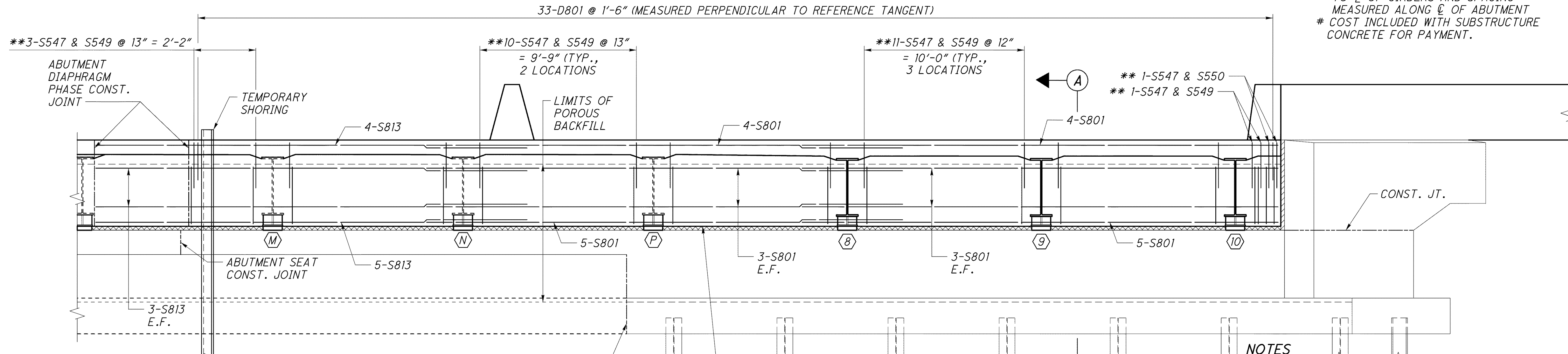
PLAN (RIGHT FORWARD ABUTMENT DIAPHRAGM) (TOP 4-#8 BARS, BOTTOM 5-#8 BARS, & SHEAR REINFORCING NOT SHOWN FOR CLARITY)
