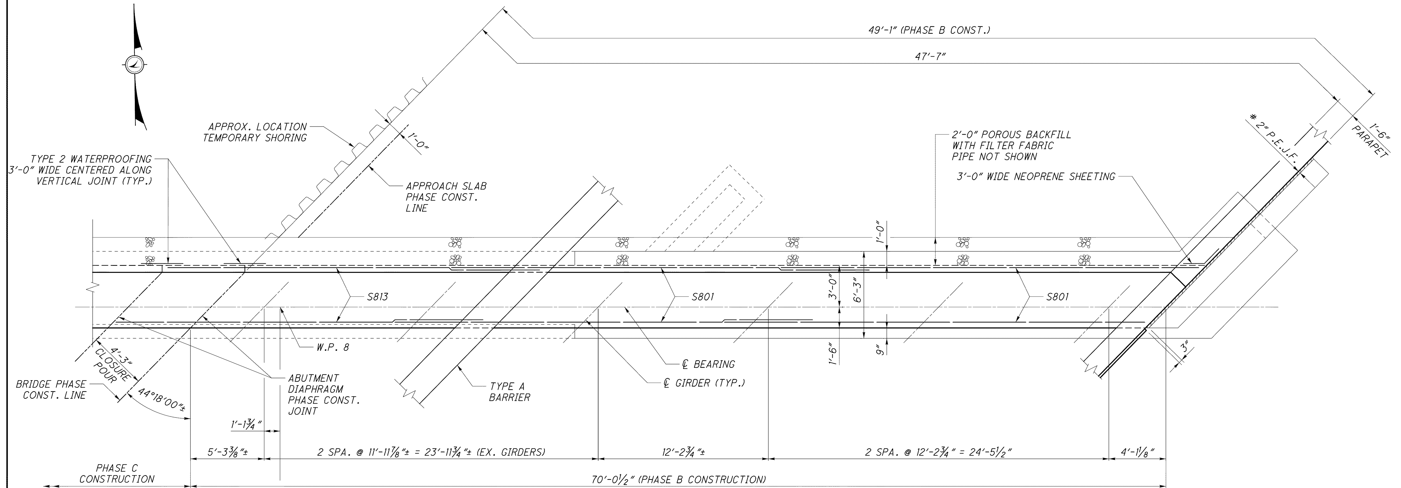
PLAN (RIGHT FORWARD ABUTMENT DIAPHRAGM) (TOP 4-#8 BARS, BOTTOM 5-#8 BARS, & SHEAR REINFORCING NOT SHOWN FOR CLARITY)
