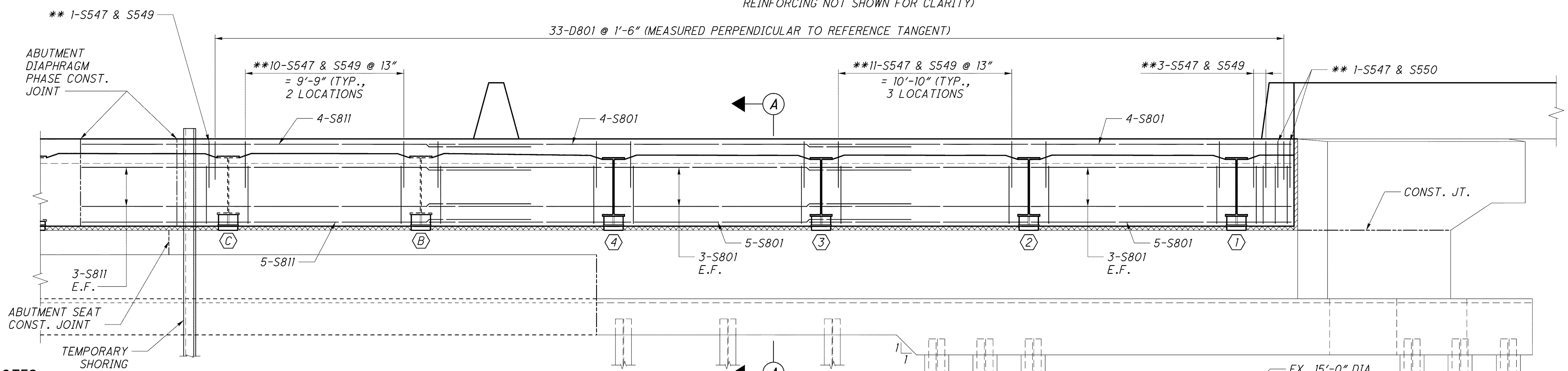
PLAN (LEFT REAR ABUTMENT DIAPHRAGM) (TOP 4-#8 BARS, BOTTOM 5-#8 BARS, & SHEAR REINFORCING NOT SHOWN FOR CLARITY)
