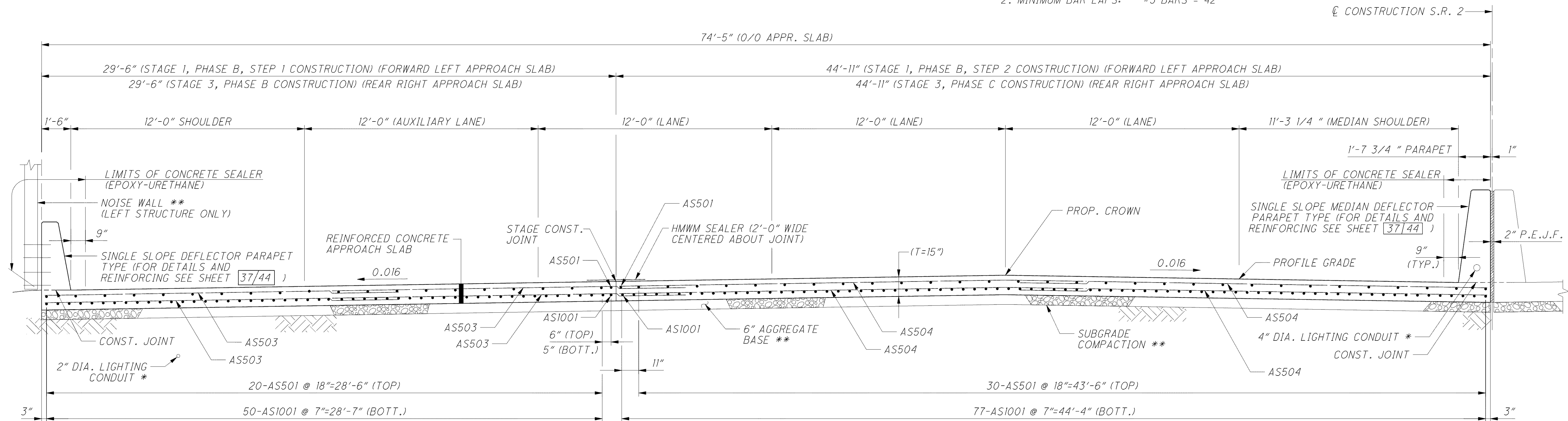
FORWARD APPROACH SLAB TRANSVERSE SECTION (LEFT STRUCTURE) (FORWARD LEFT APPROACH SLAB SHOWN, REAR RIGHT APPROACH SLAB SIMILAR)
