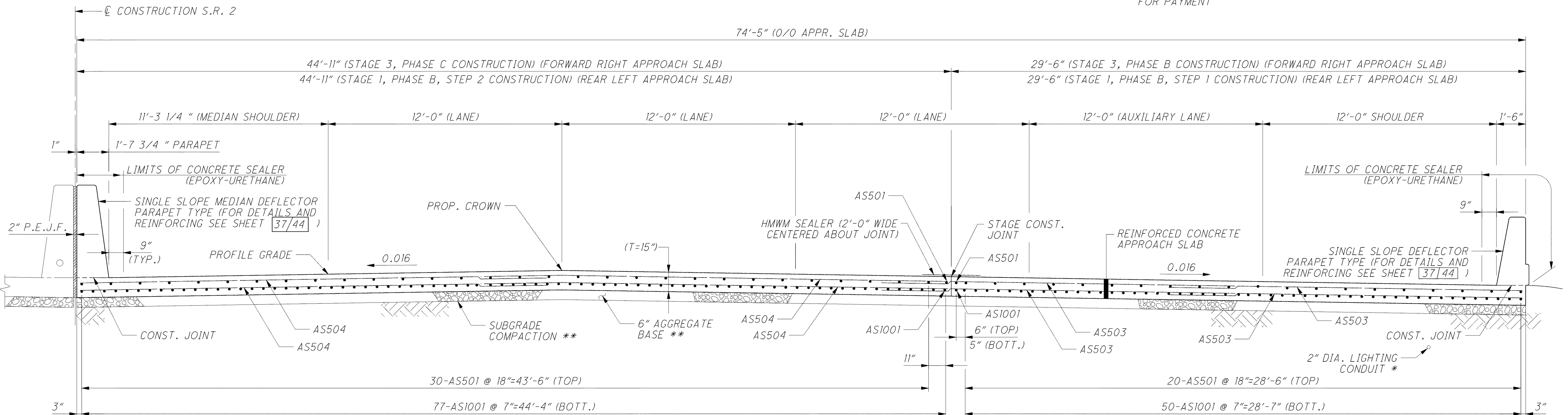
FORWARD APPROACH SLAB TRANSVERSE SECTION (RIGHT STRUCTURE) (FORWARD RIGHT APPROACH SLAB SHOWN, REAR LEFT APPROACH SLAB SIMILAR)
