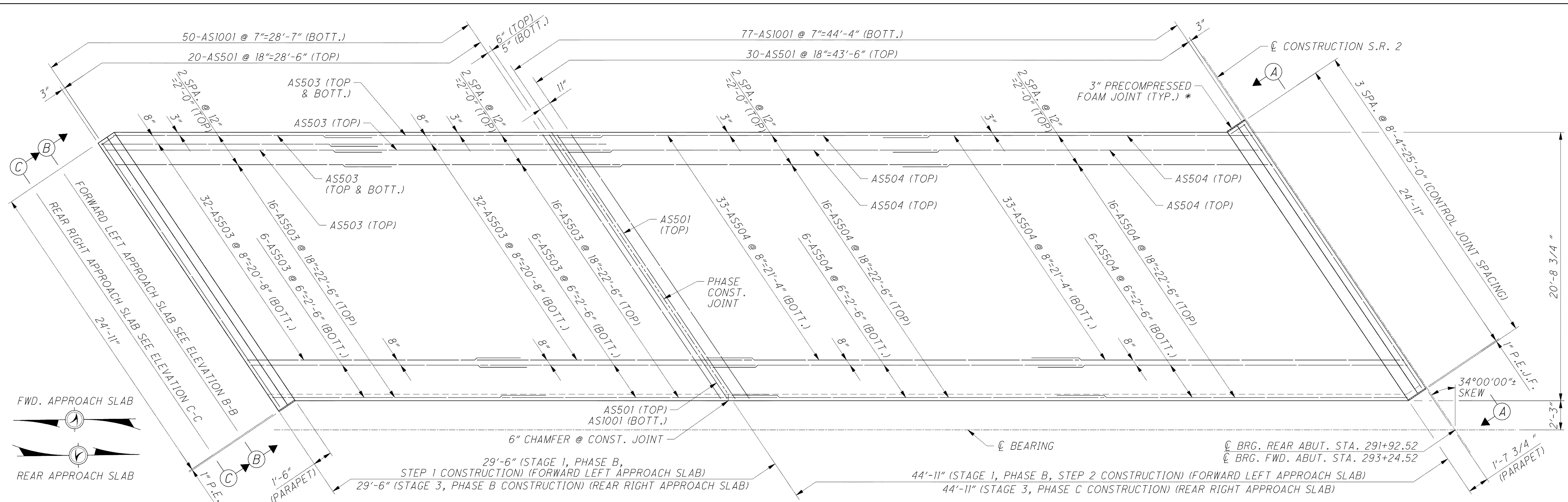
FORWARD APPROACH SLAB PLAN (LEFT STRUCTURE) (FORWARD LEFT APPROACH SLAB SHOWN, REAR RIGHT APPROACH SLAB SIMILAR)
