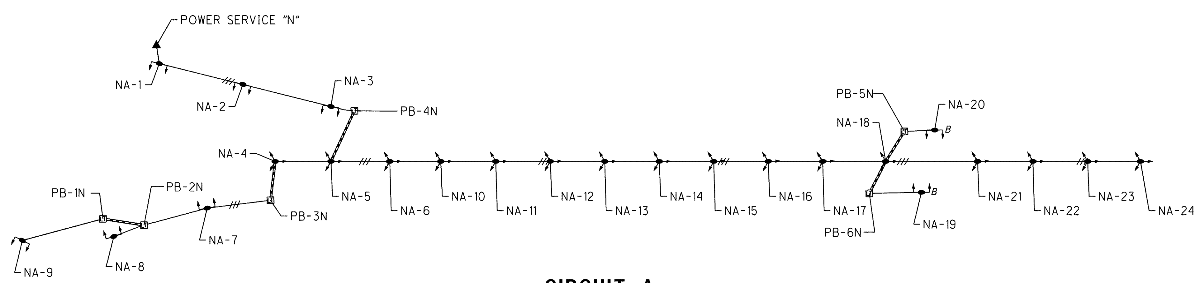
CIRCUIT A POWER SERVICE "N"
