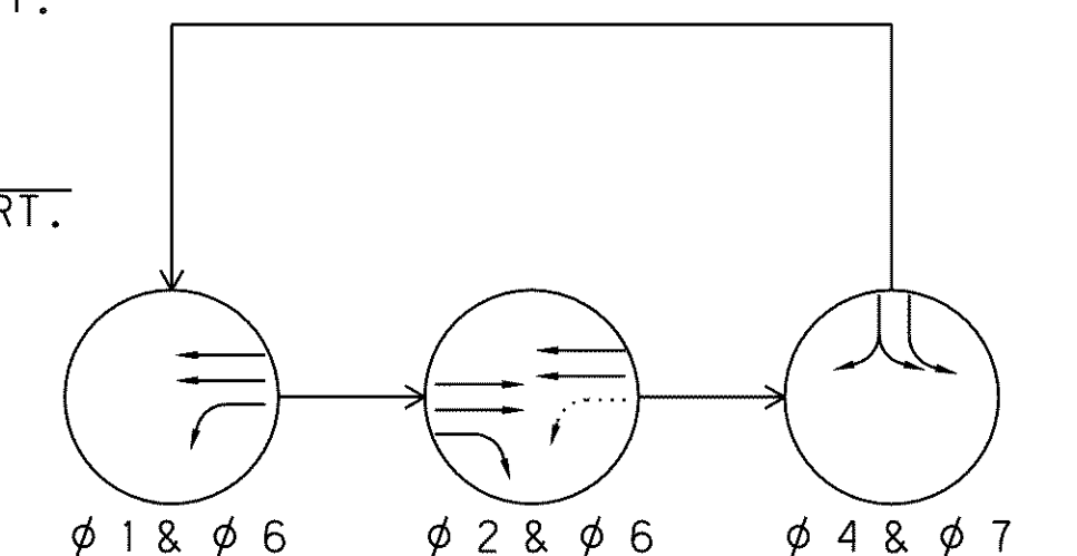
PHASING DIAGRAM
