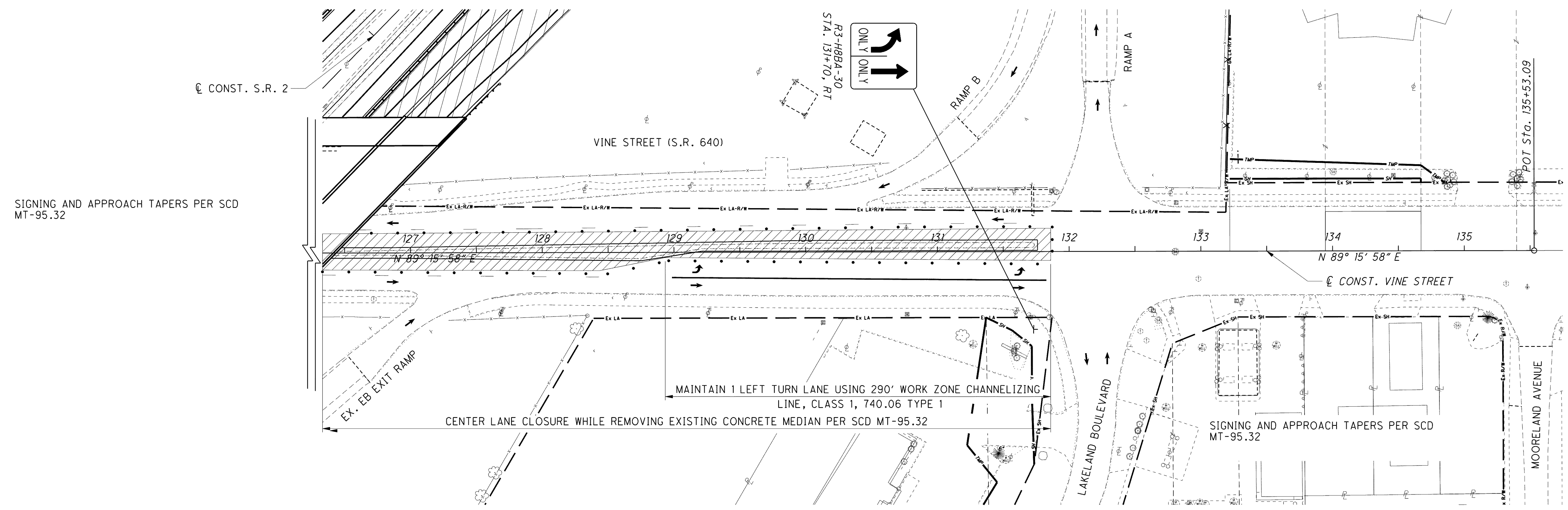
PHASE B STEP 3 - REMOVAL OF EXISTING CONCRETE MEDIAN
