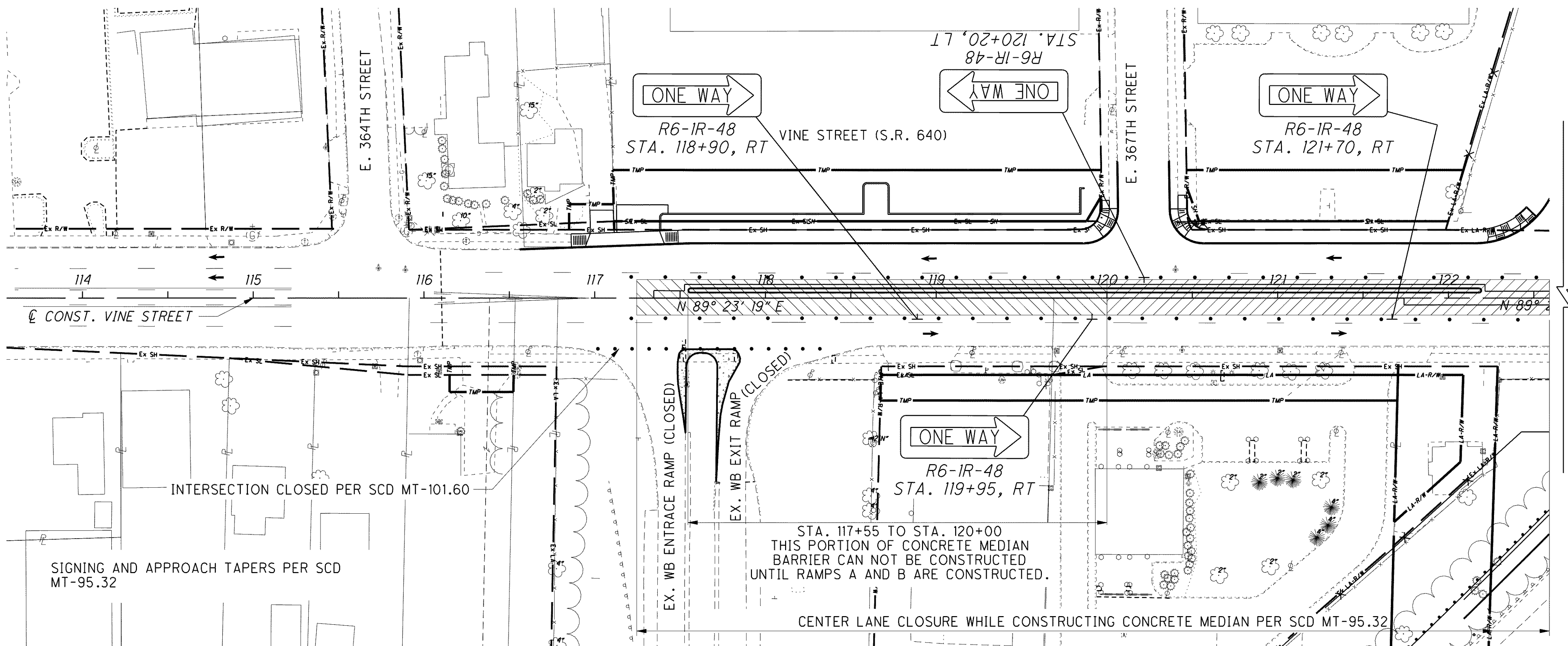
PHASE B STEP 4 - CONSTRUCTION OF PROPOSED CONCRETE MEDIAN
