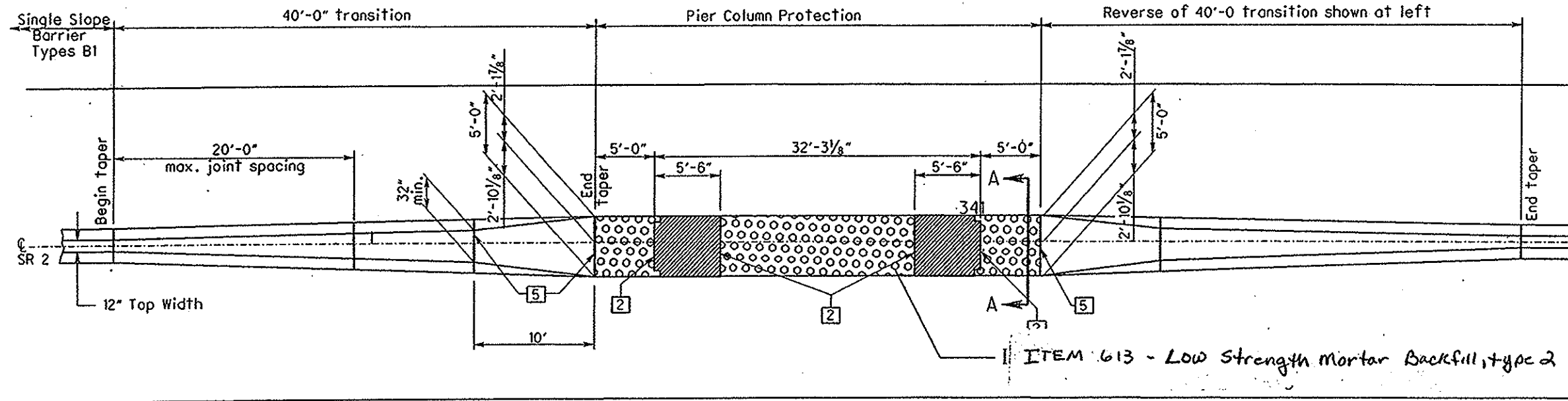
PLAN VIEW - BRIDGE PIER TRANSITION @ CSX RR
