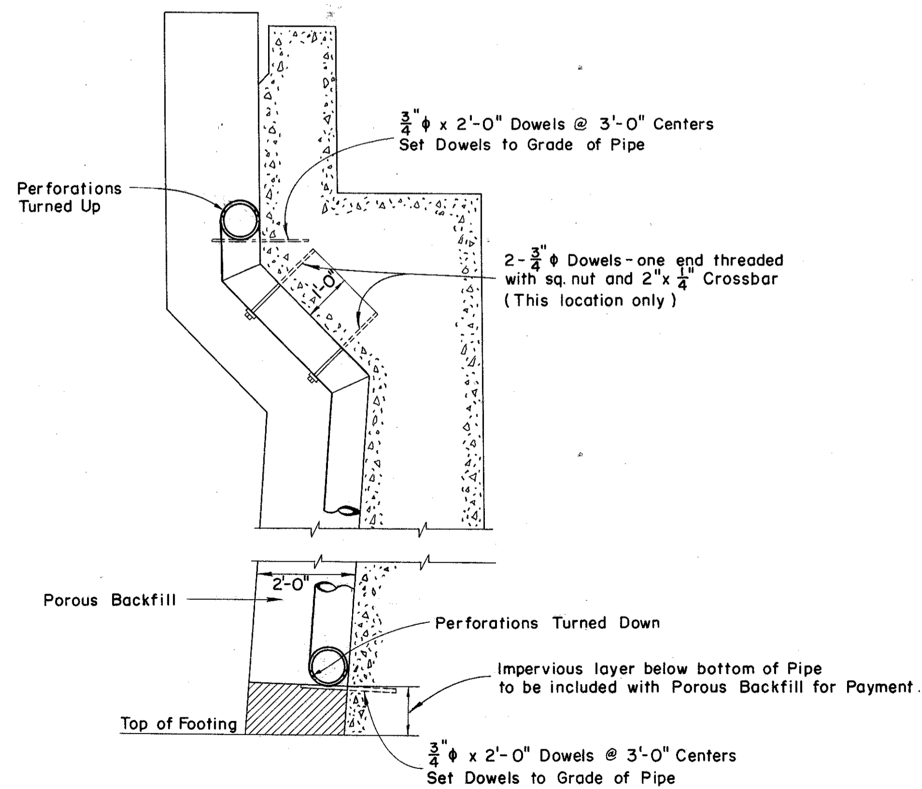
DRAIN DETAILS
