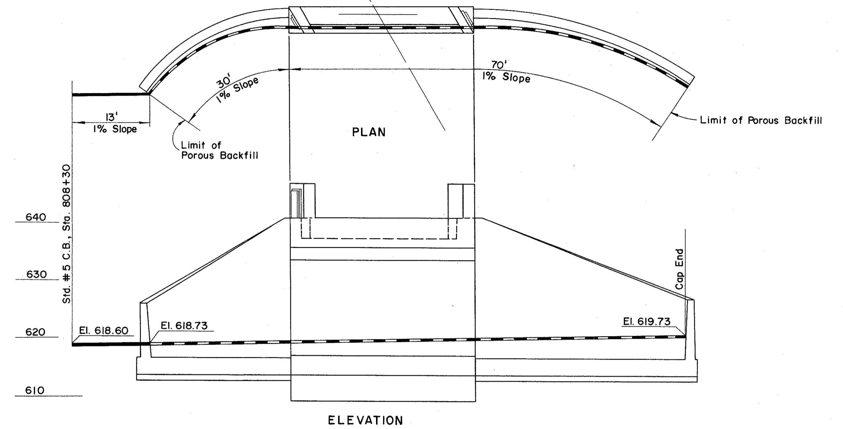
DRAINAGE OF REAR ABUTMENT
