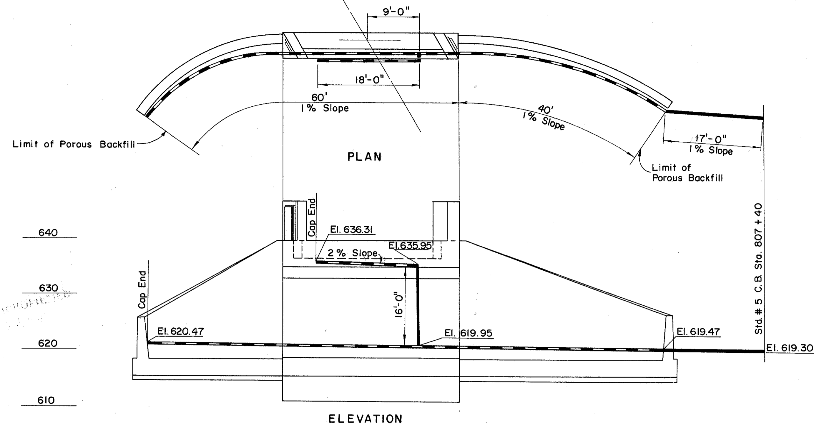
DRAINAGE OF FORWARD ABUTMENT
