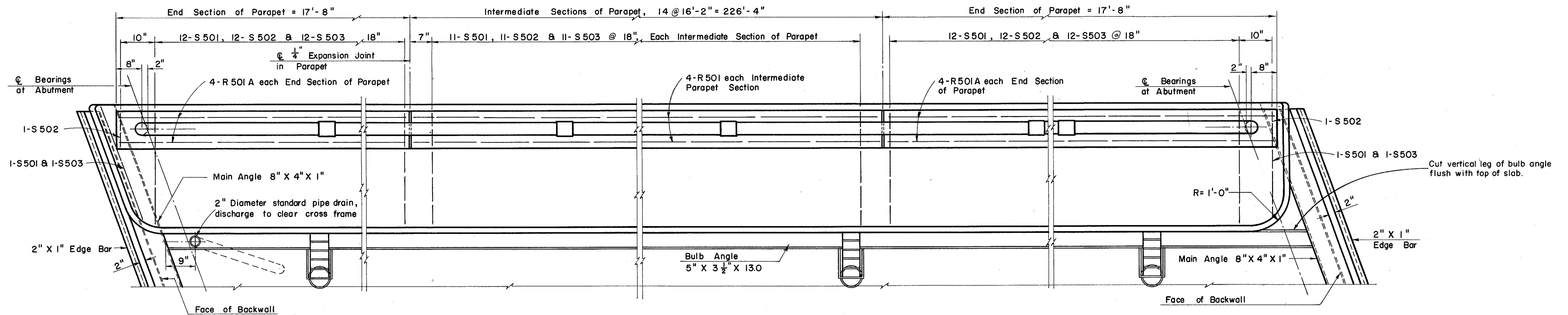
PARAPET & CURB REINFORCEMENT PLAN
