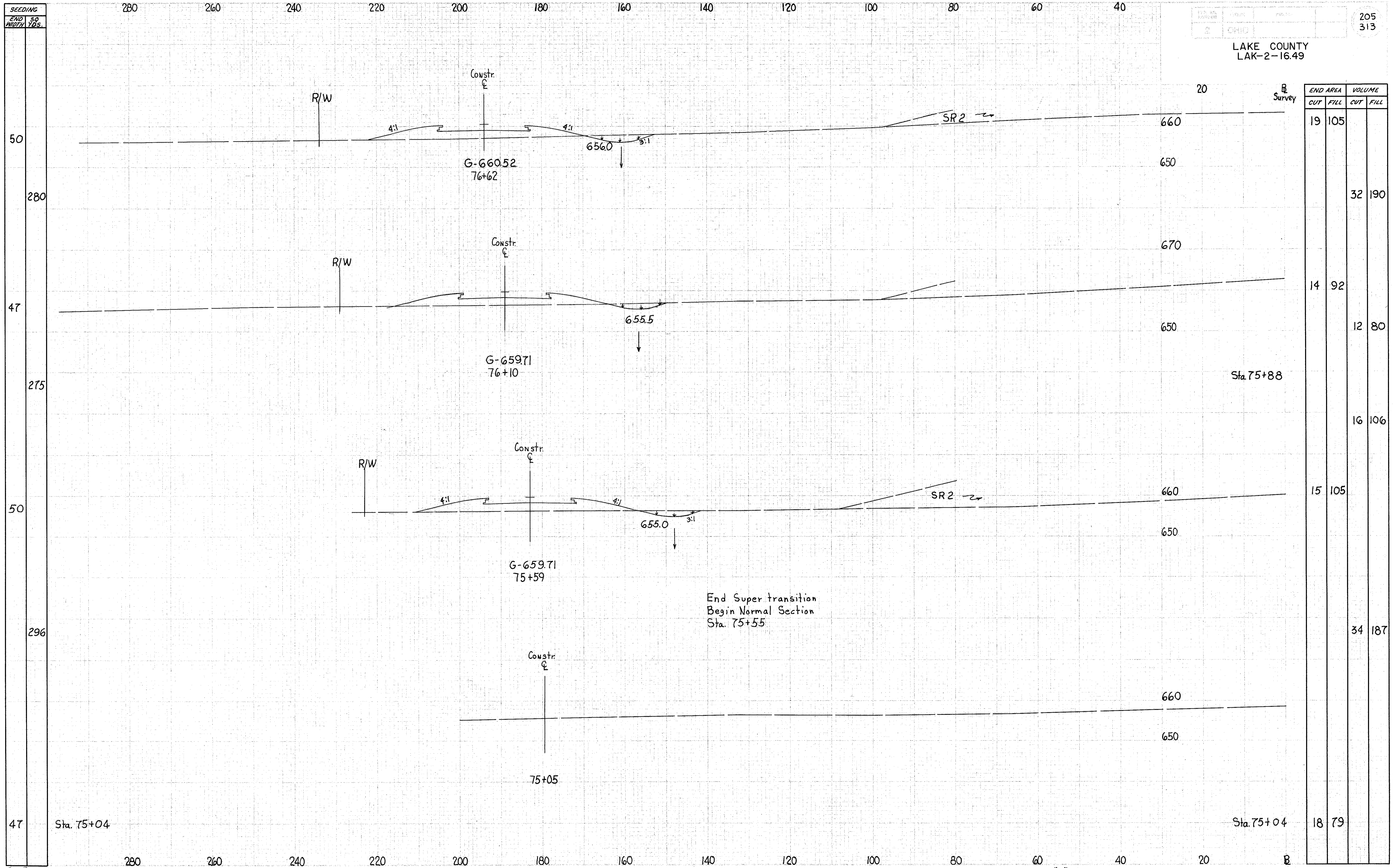
FRONTAGE ROAD "B" Sta. 75+05 to Sta. 76+62
