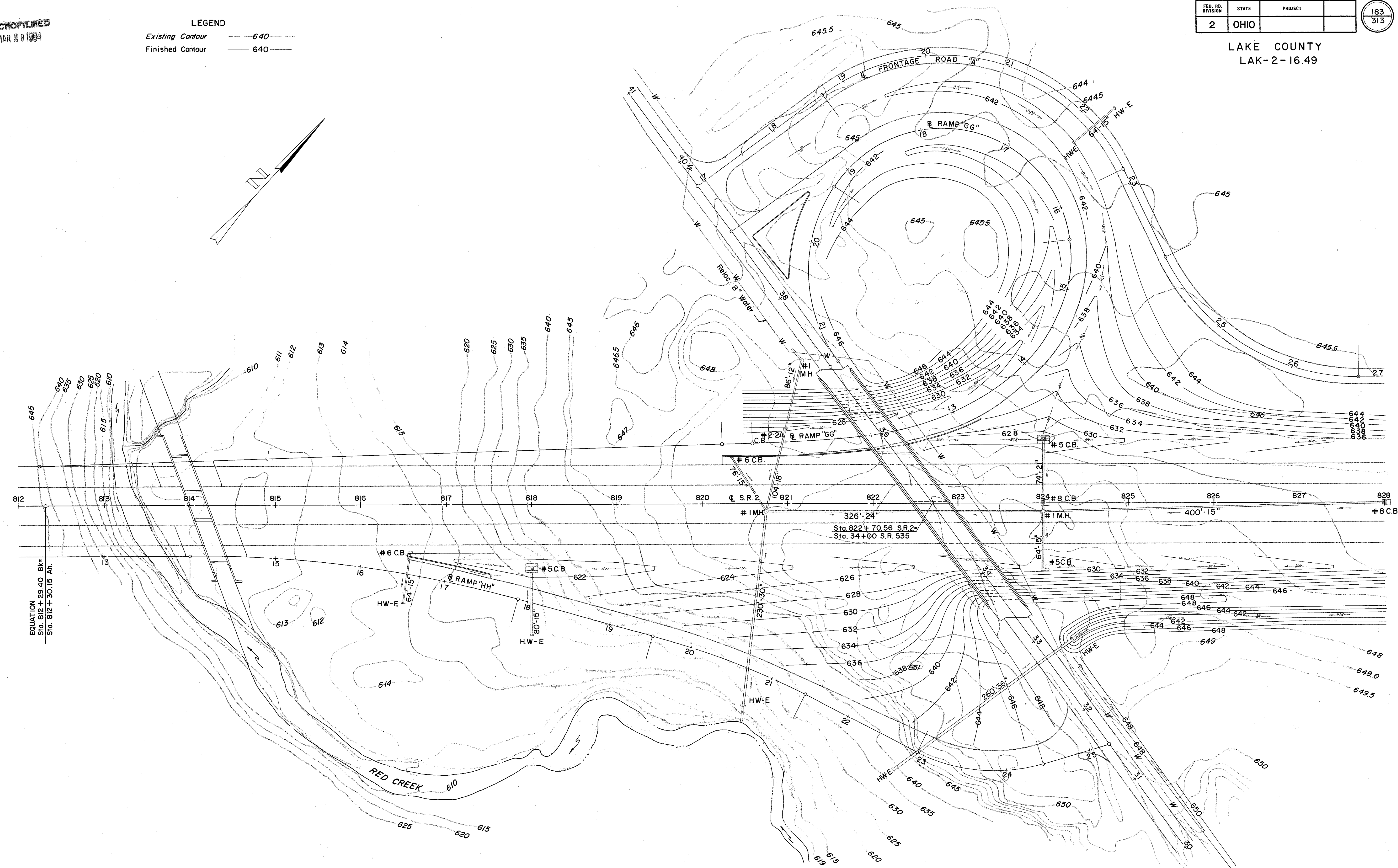
S.R. 535 INTERCHANGE GRADING PLAN
