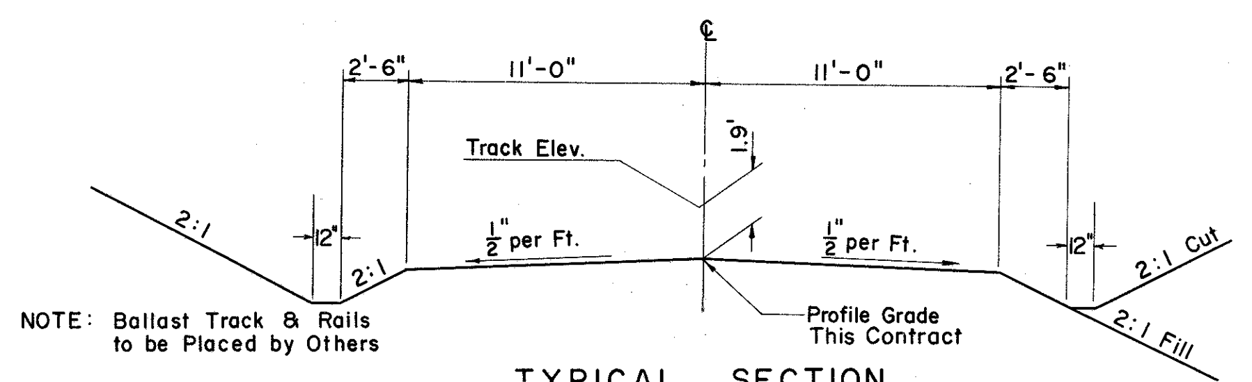
TYPICAL SECTION F.P. & E. RAILROAD TEMP. RUNAROUND
