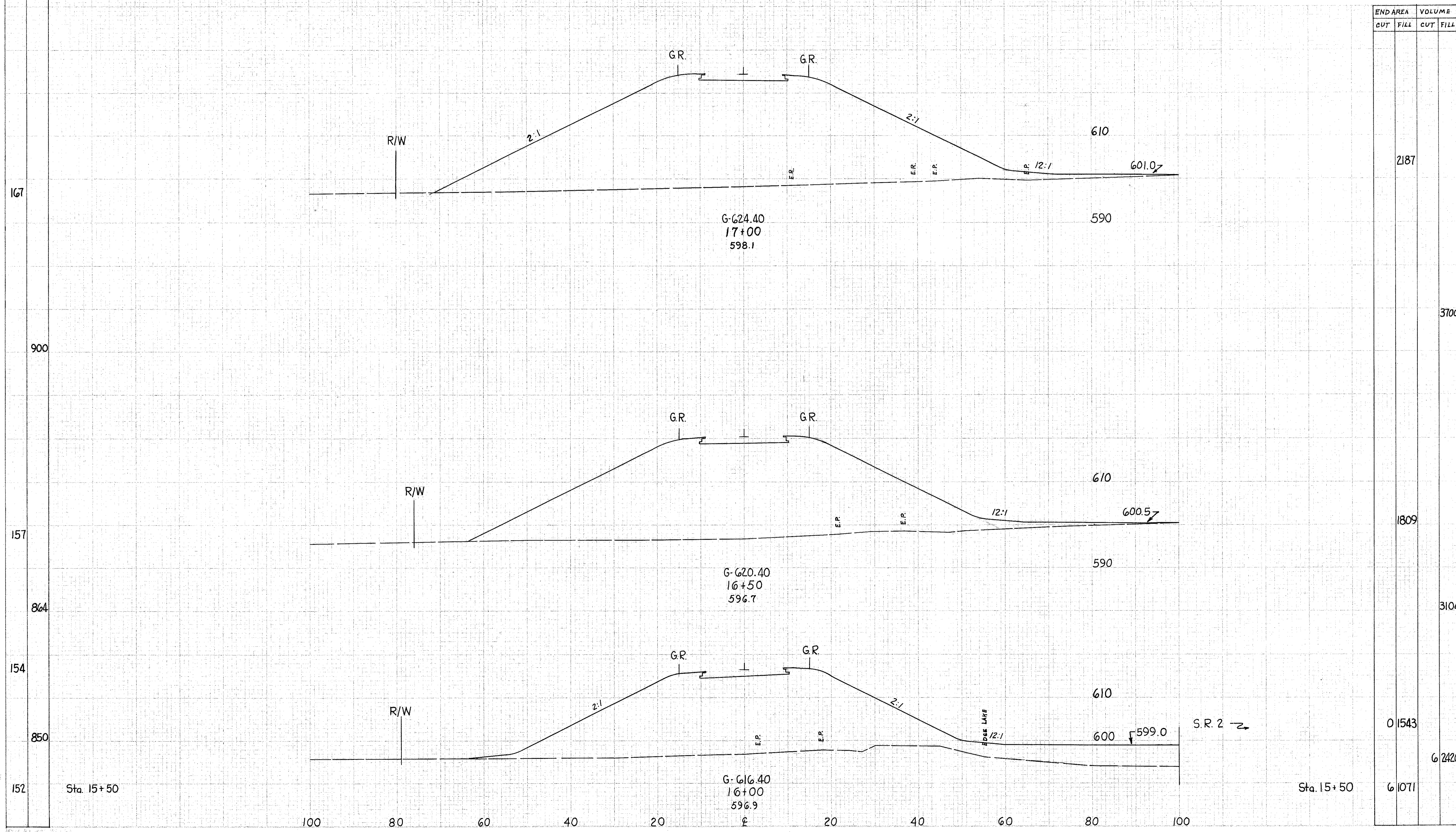
RELOCATION RIVER ROAD Sta. 16+00 to 17+00
