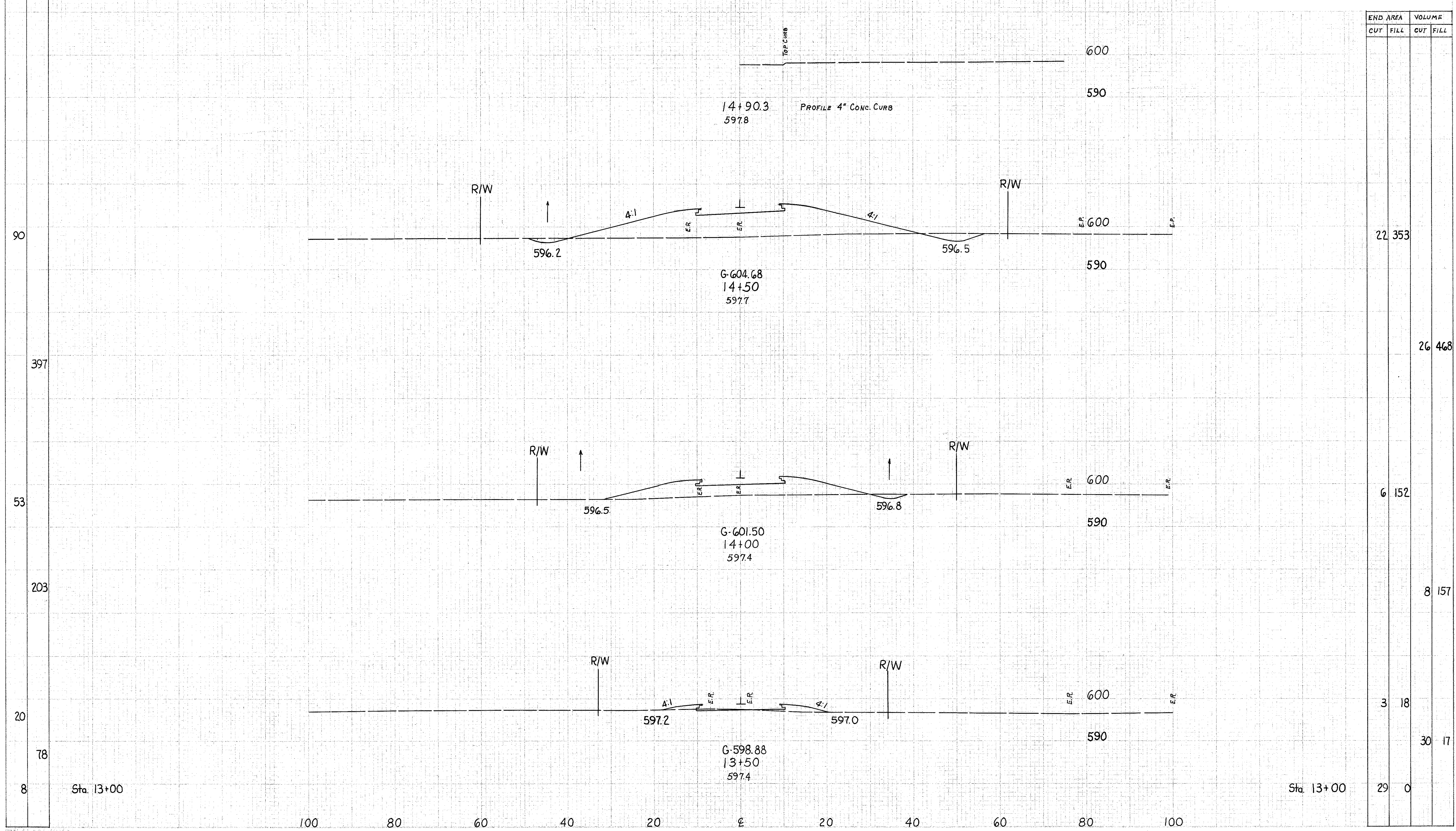
RELOCATION RIVER ROAD Sta. 13+50 to 14+90.3
