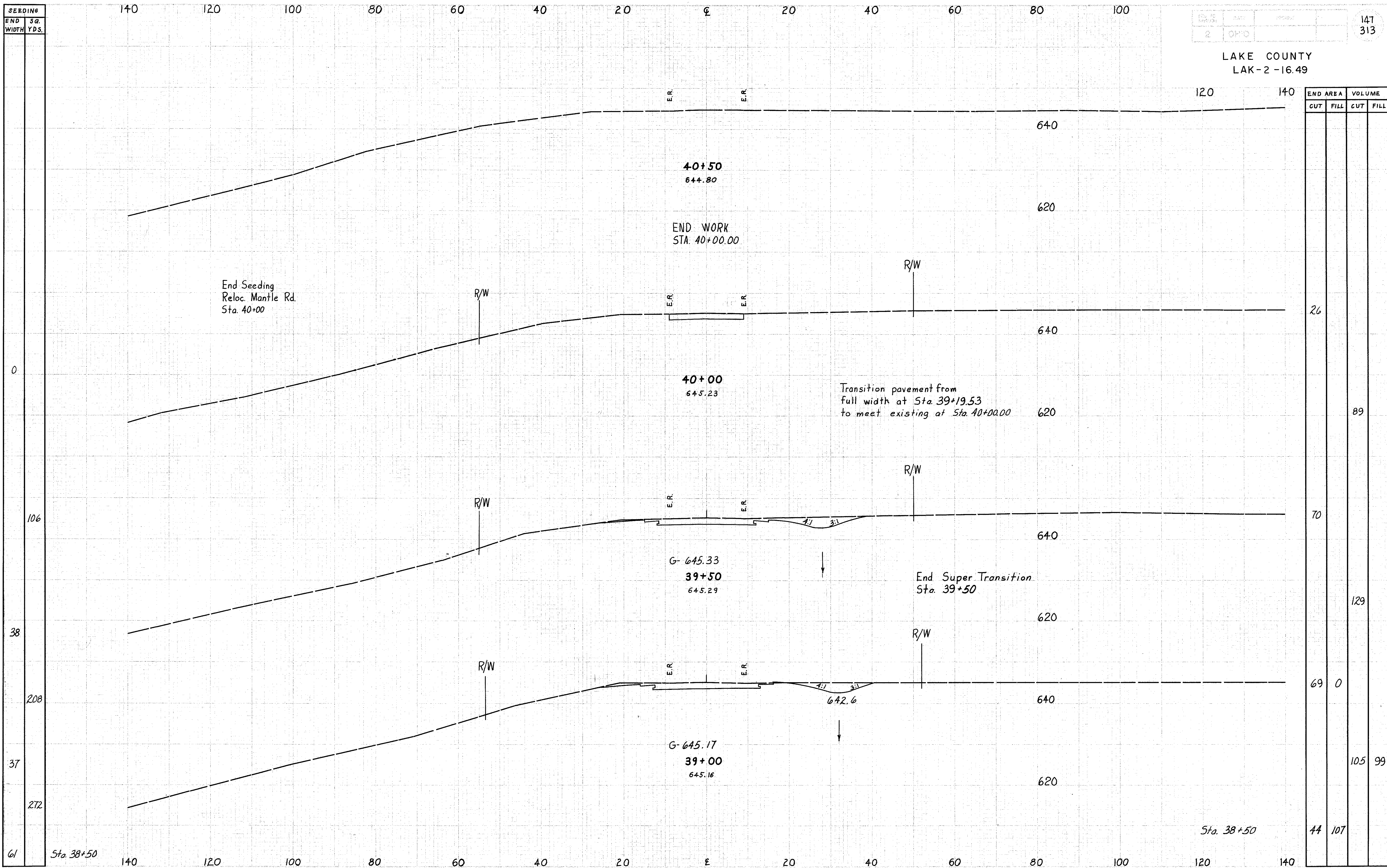
RELOCATION MANTLE ROAD STA. 39+00 to 40+50
