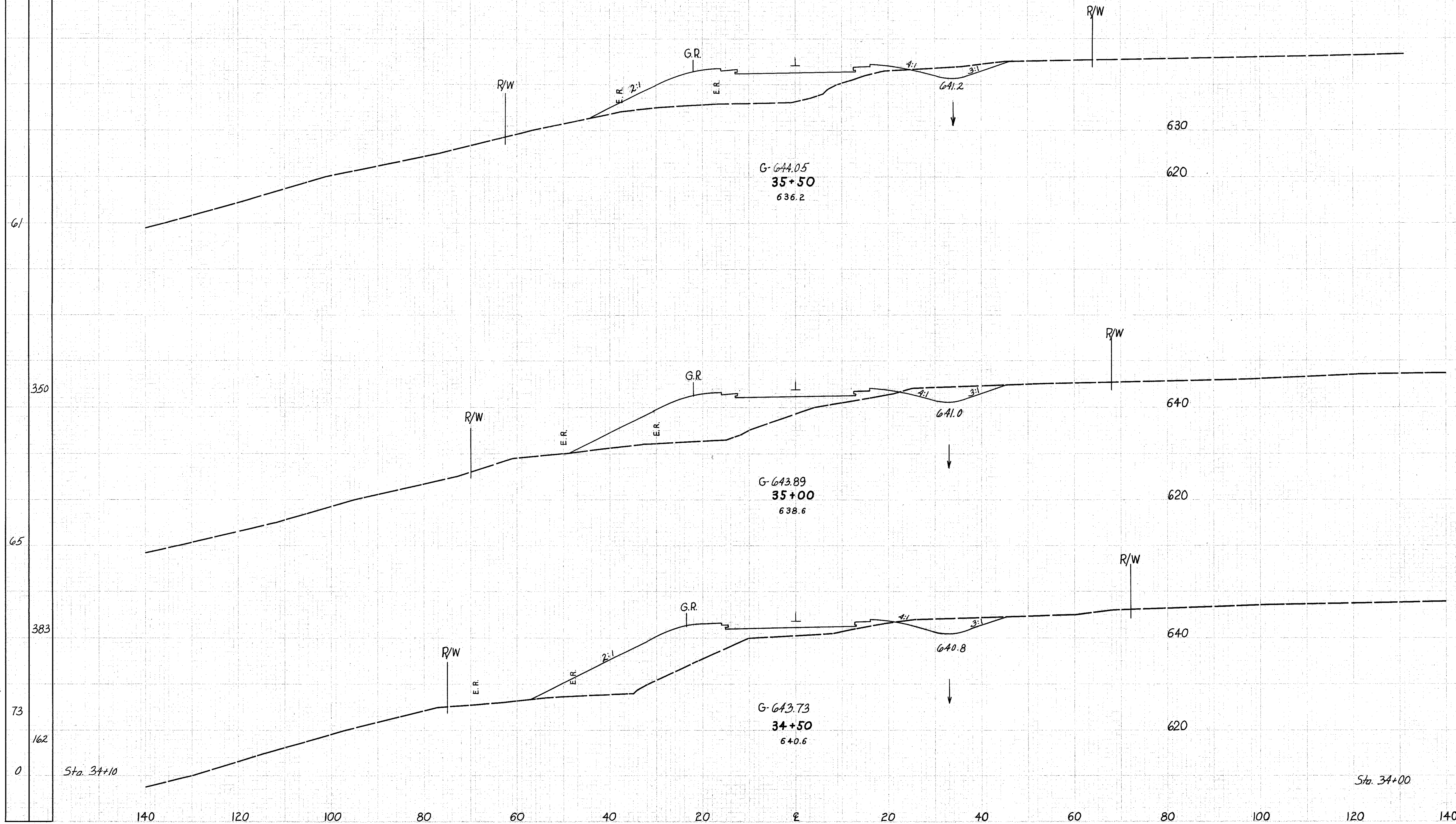
RELOCATION MANTLE ROAD STA. 34+50 to 35+50
