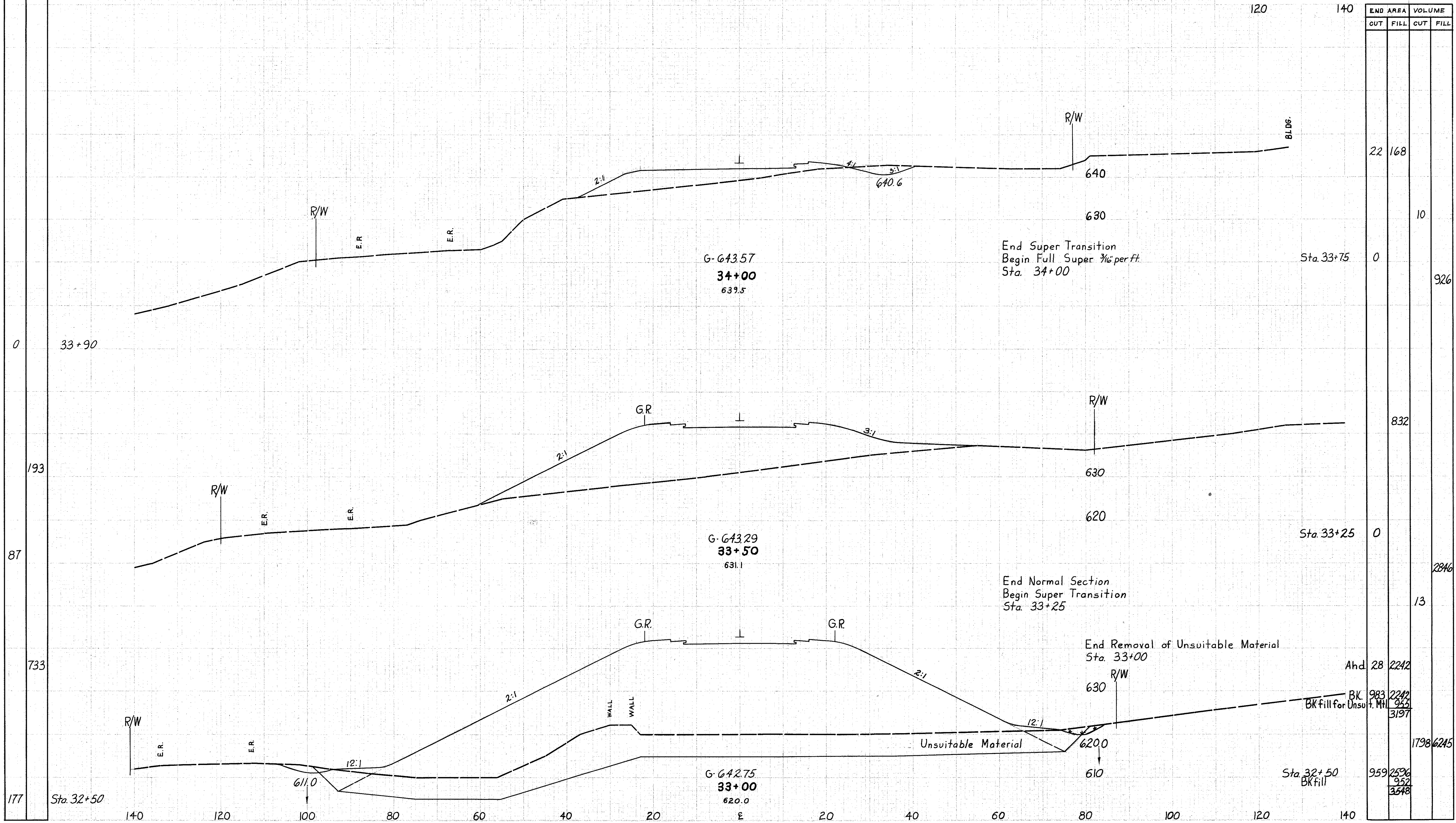
RELOCATION MANTLE ROAD STA. 33+00 to 34+00
