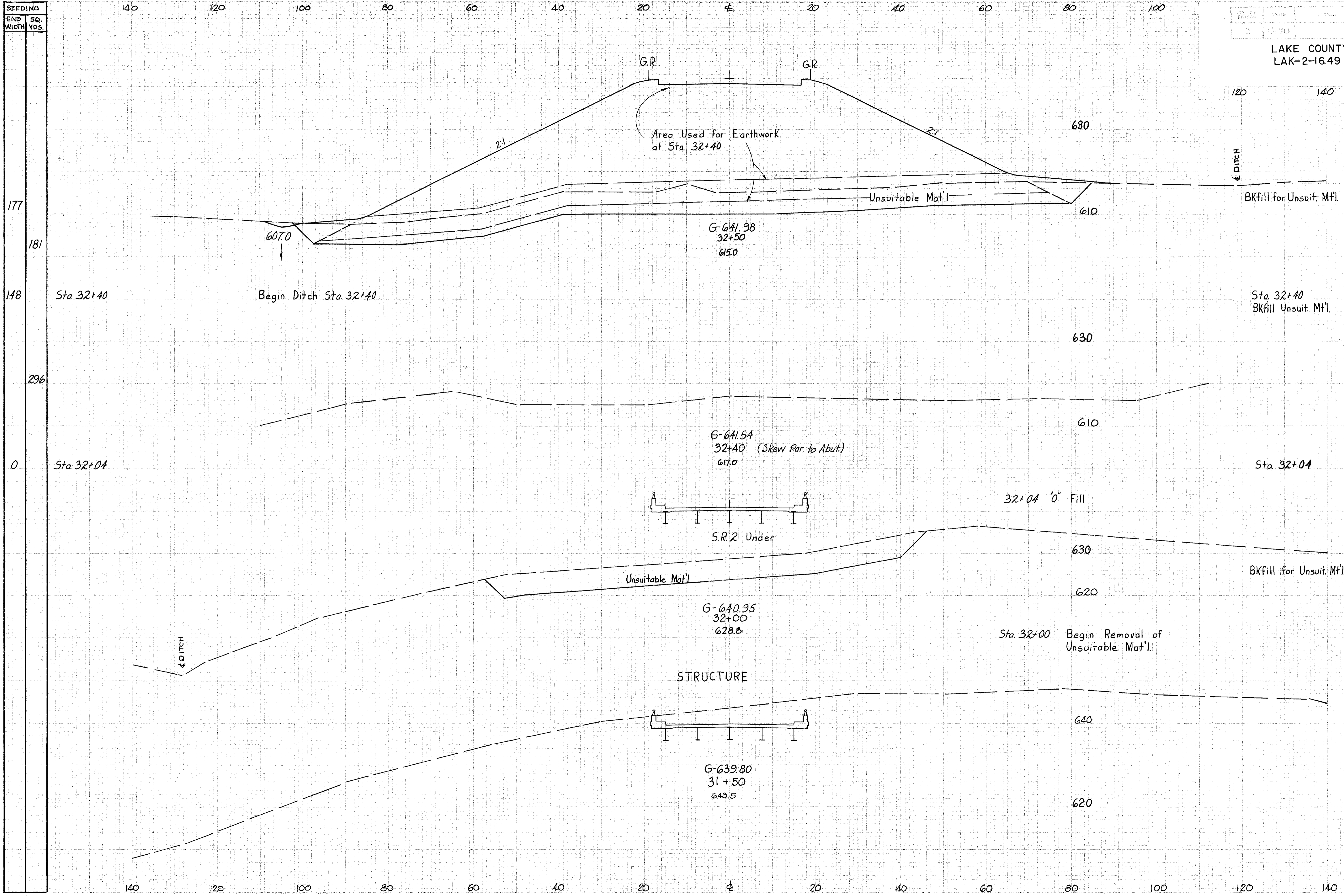
RELOCATION MANTLE ROAD STA. 31+50 to 32+50
