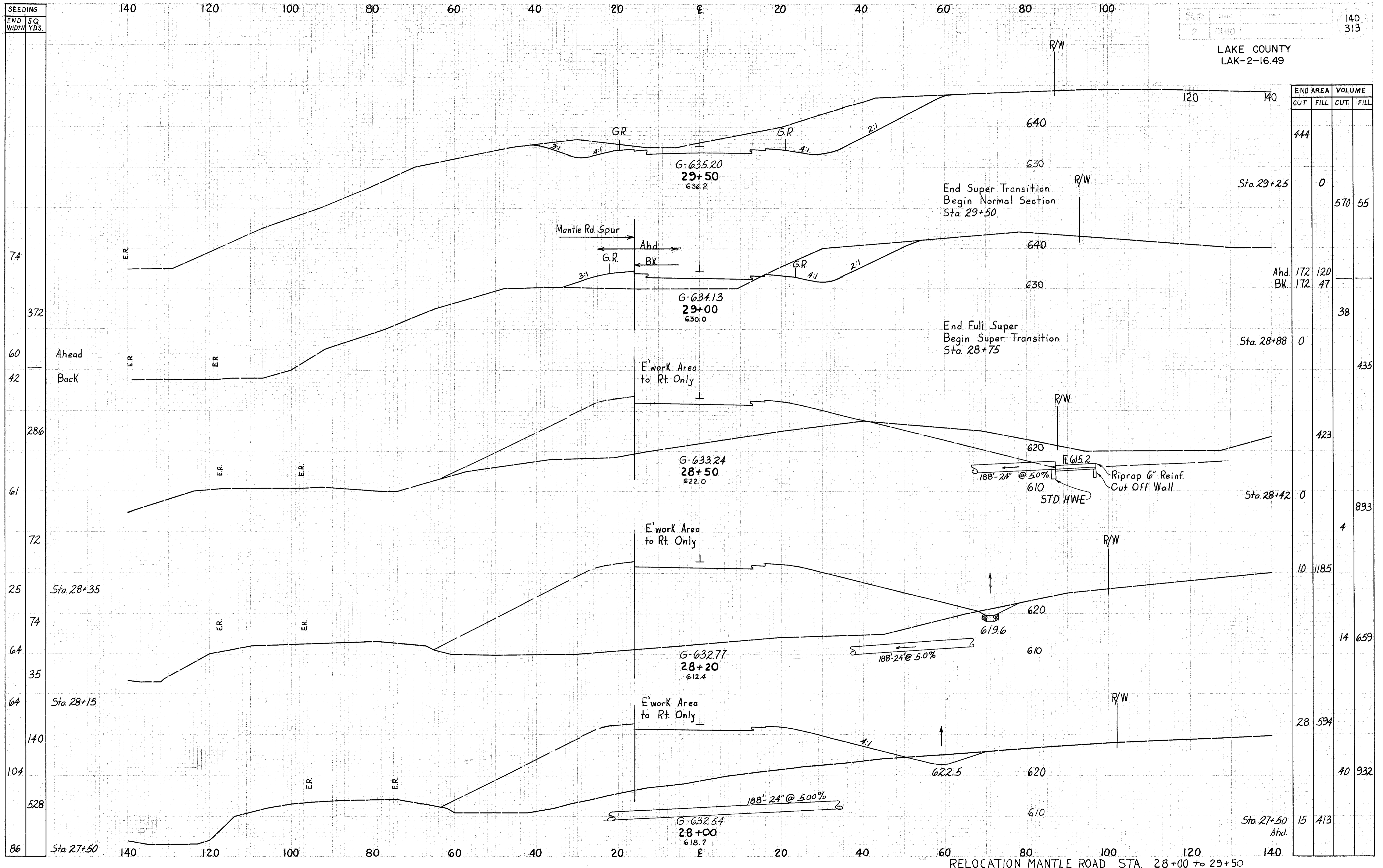
RELOCATION MANTLE ROAD STA. 28+00 TO 29+50
