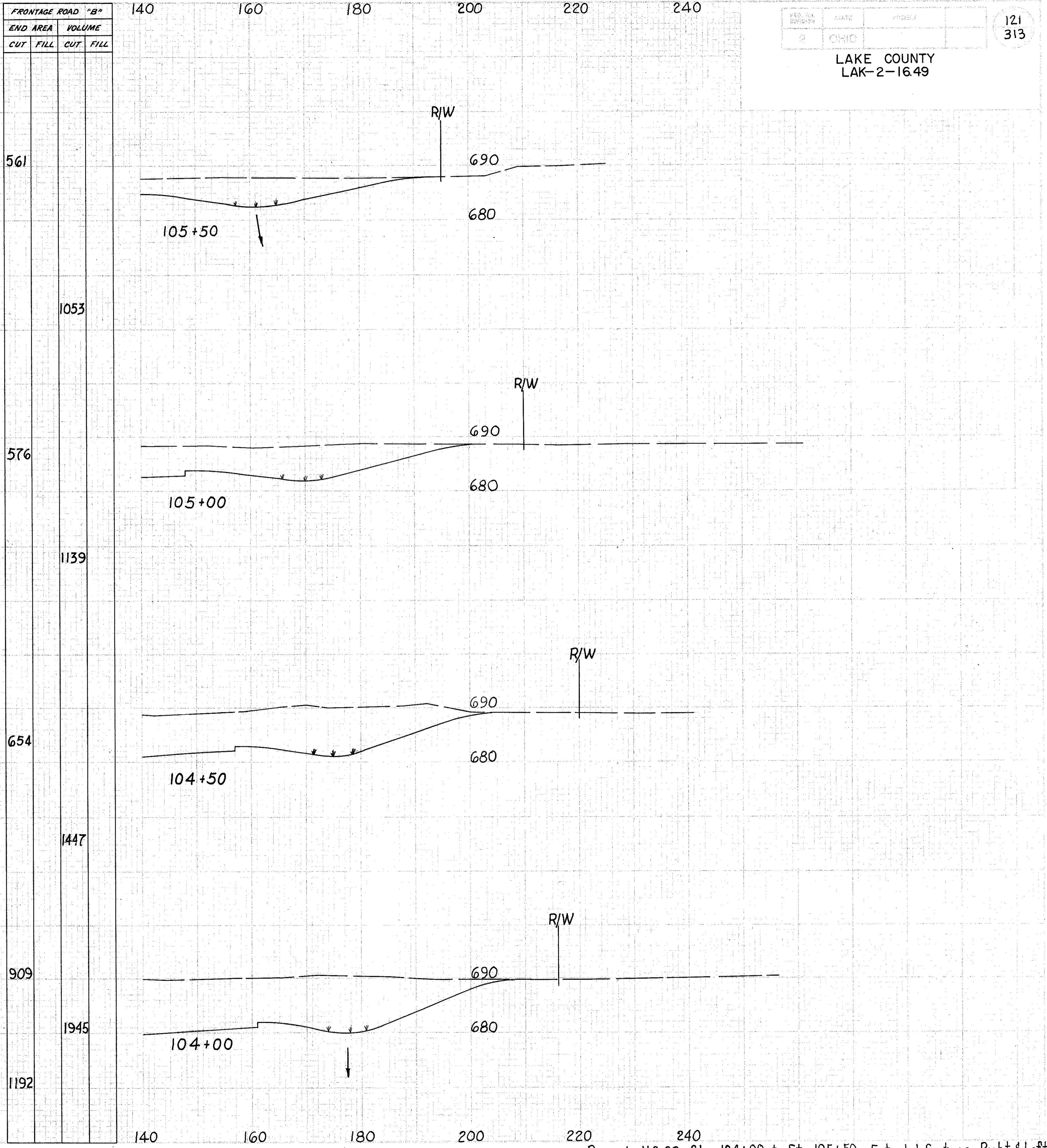
Reconstr. U.S. 20 Sta 104+00 to Sta 105+50 Extended Sections, Right & Left
