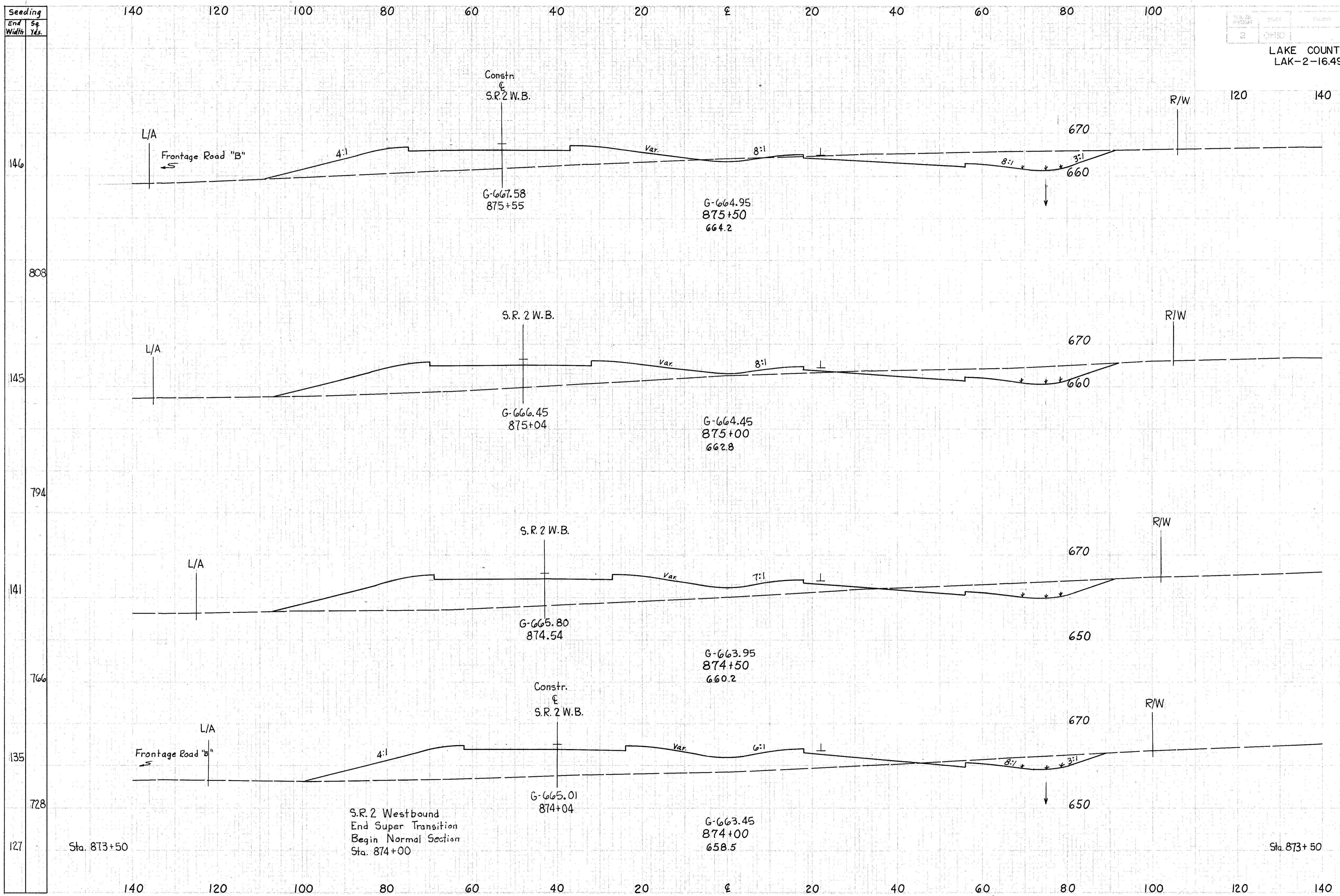
RELOCATION S.R. 2 Sta 874+00 to 875+50
