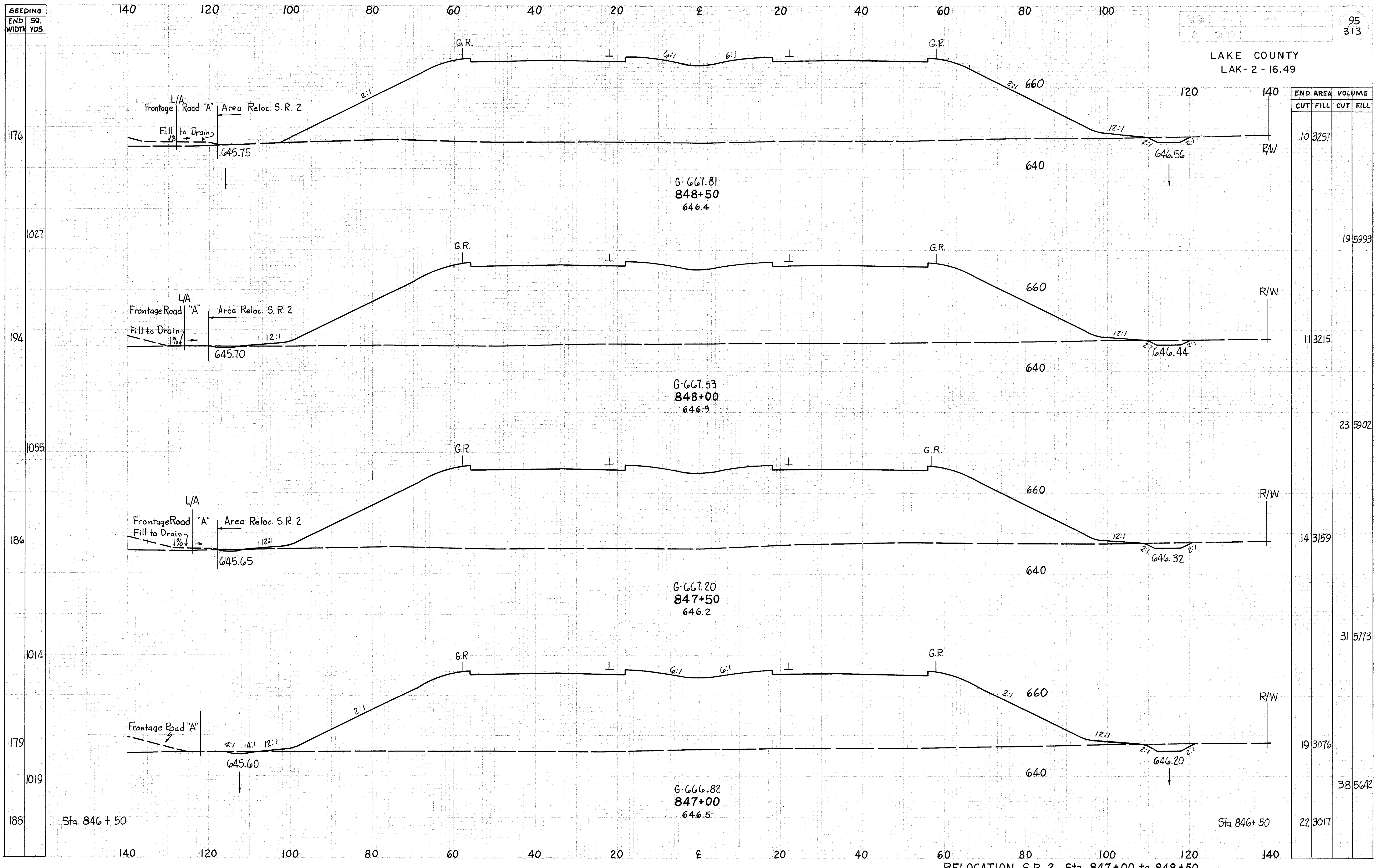
RELOCATION S.R. 2 Sta. 847+00 to 848+50
