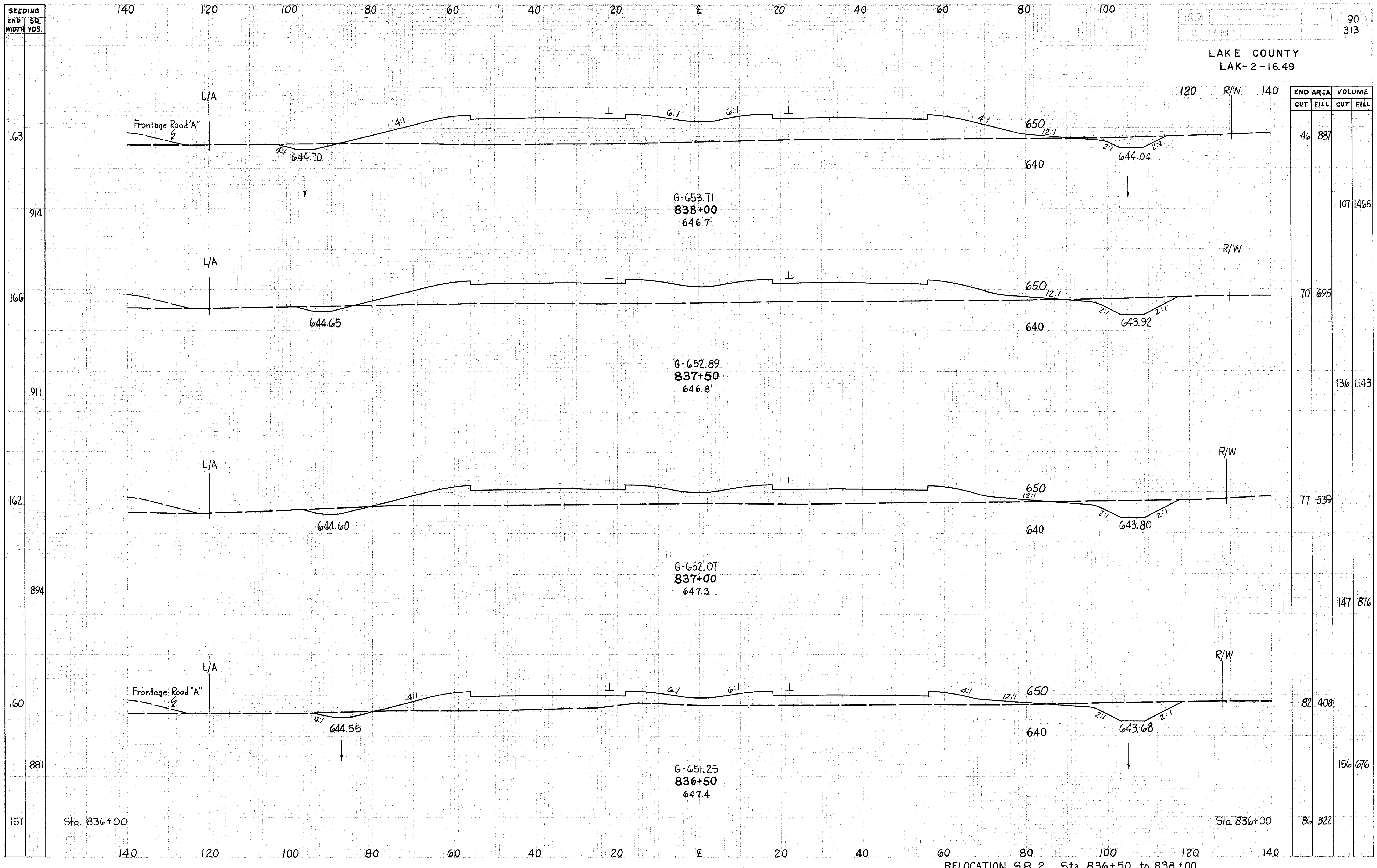
RELOCATION S.R. 2 Sta. 836+50 to 838+00
