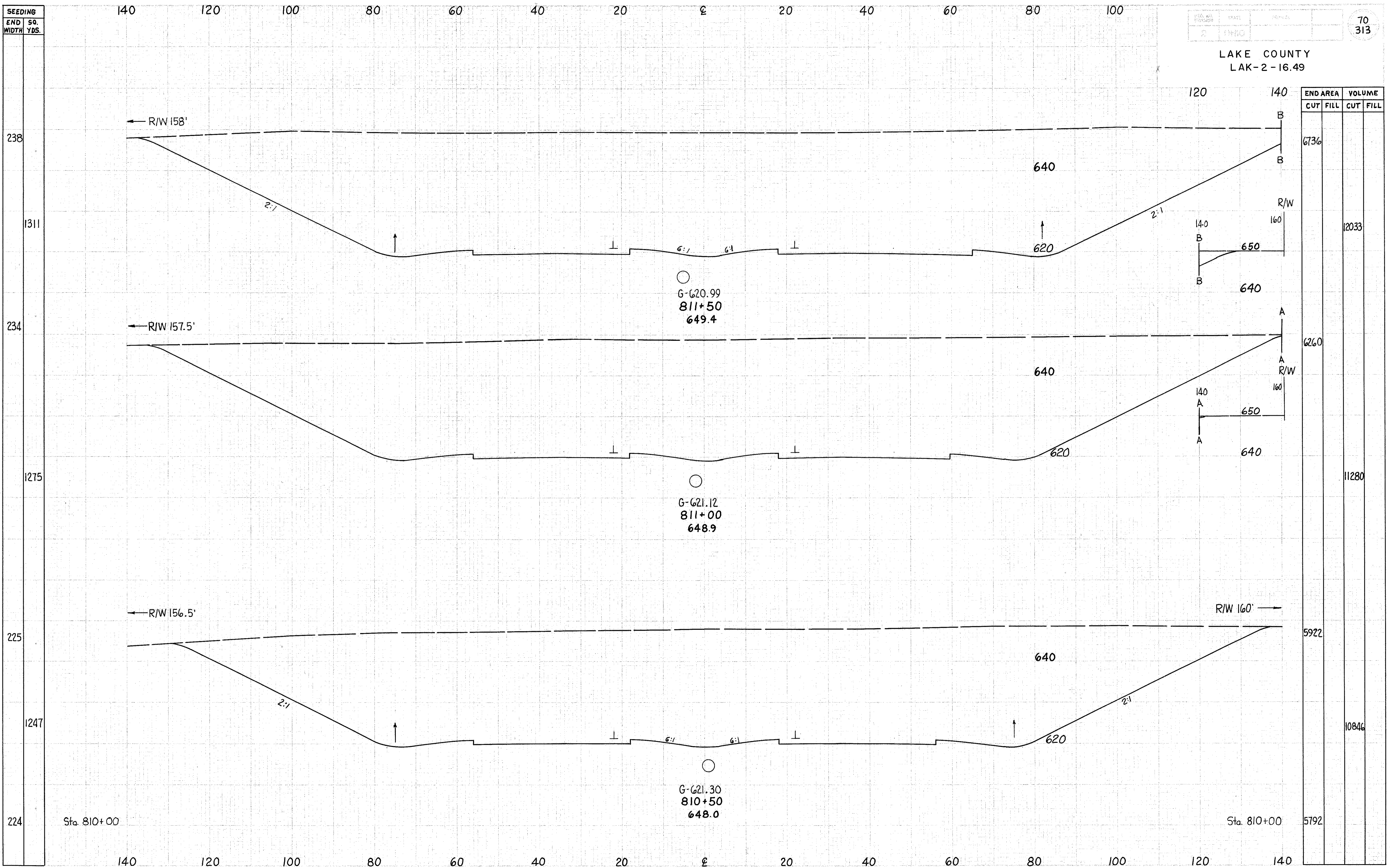
RELOCATION S.R.2 Sta. 810+50 to 811+50
