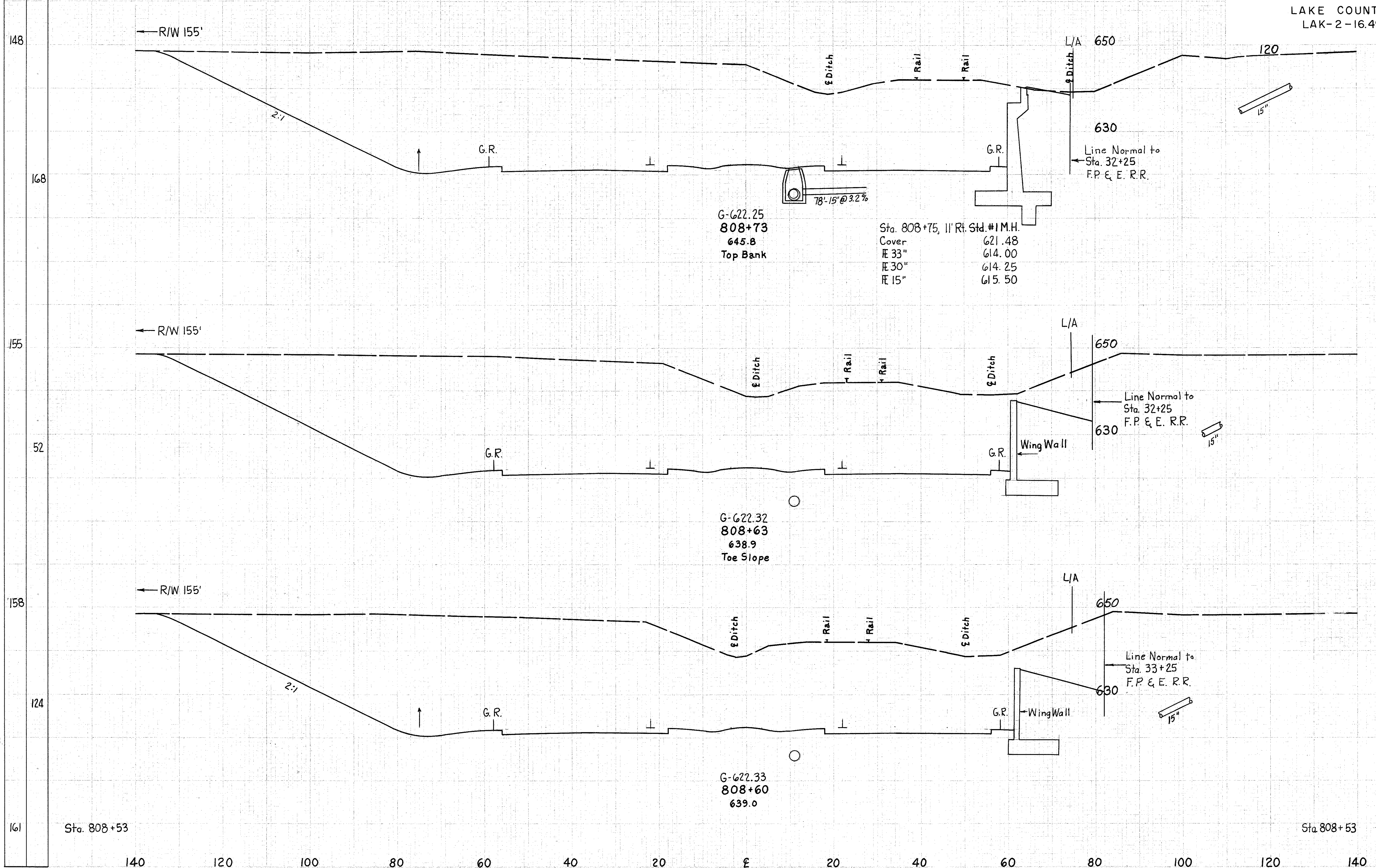
RELOCATION S.R.2 Sta. 808+60 to 808+73
