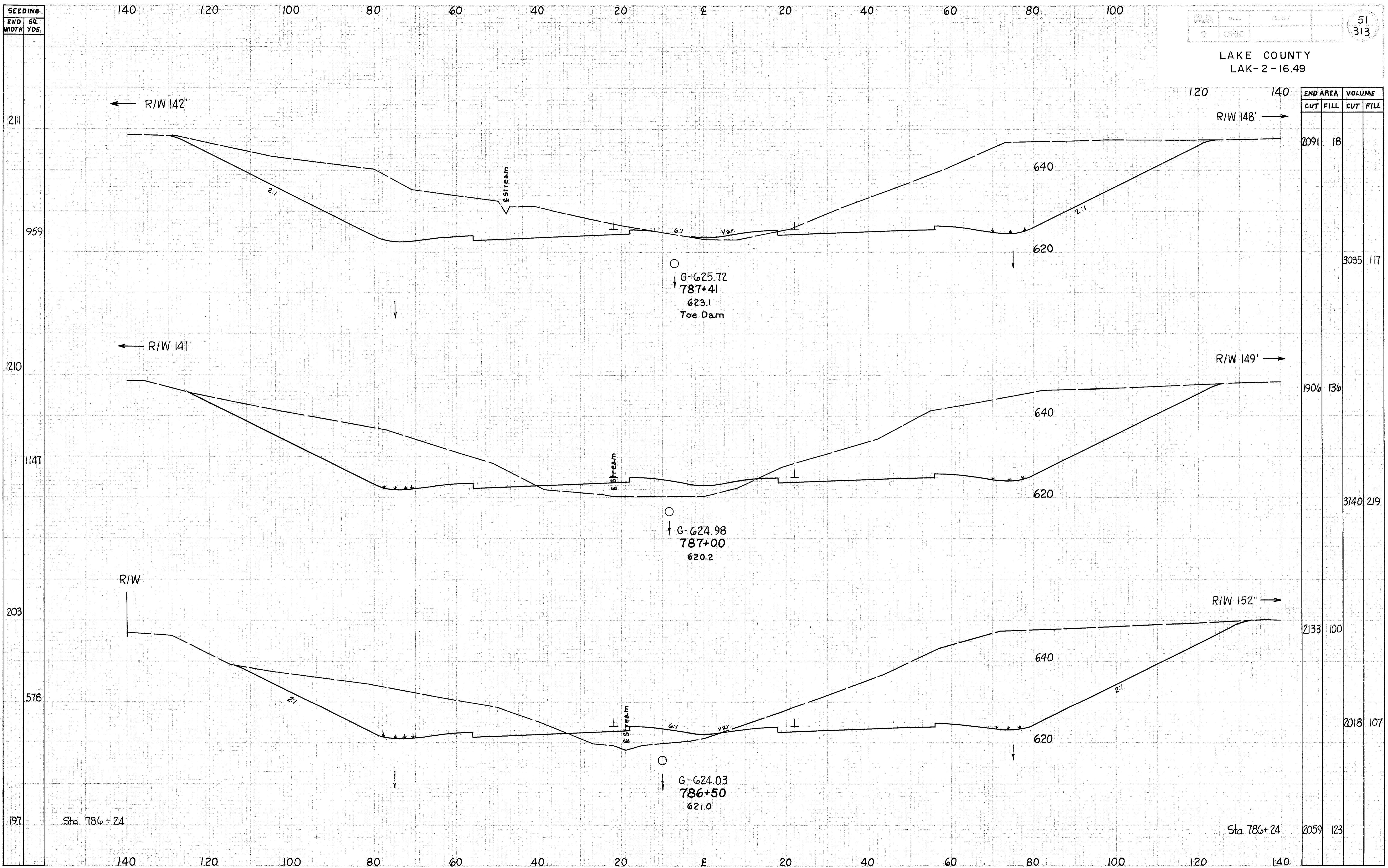
RELOCATION S.R. 2 Sta. 786+50 to 787+41
