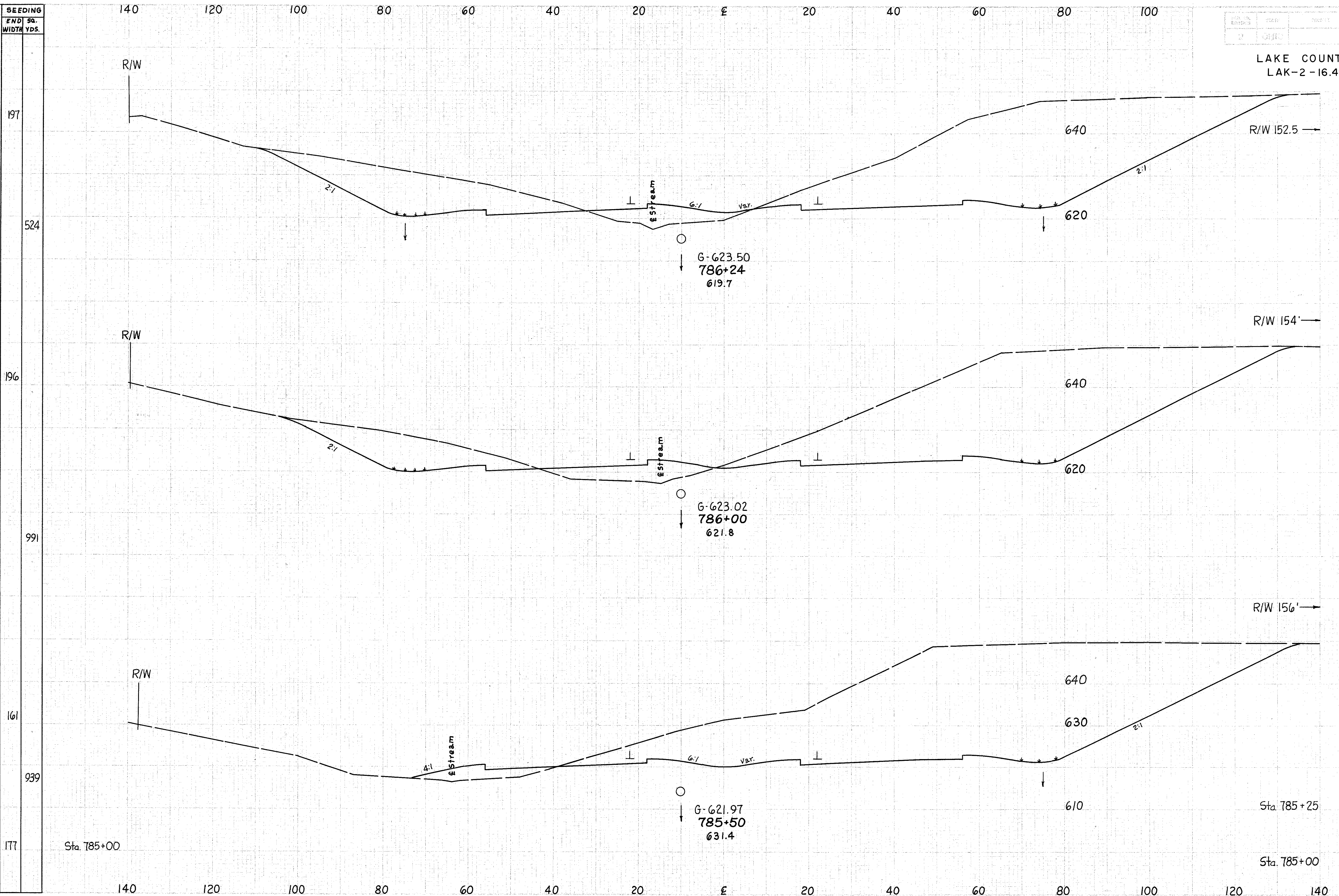
RELOCATION S.R.2 Sta. 785+50 to 786+24
