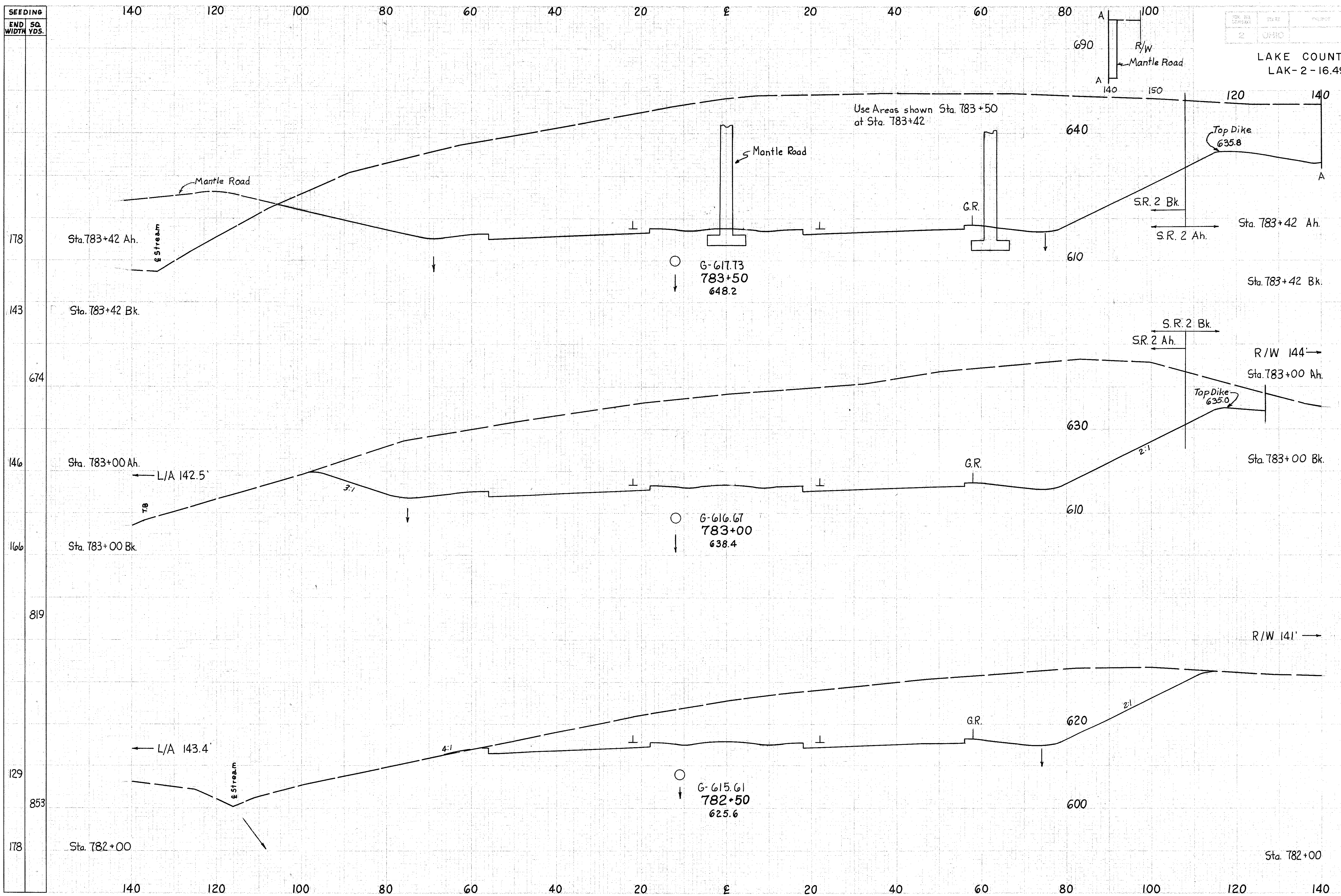
RELOCATION S.R. 2 Sta. 782+50 to 783+50
