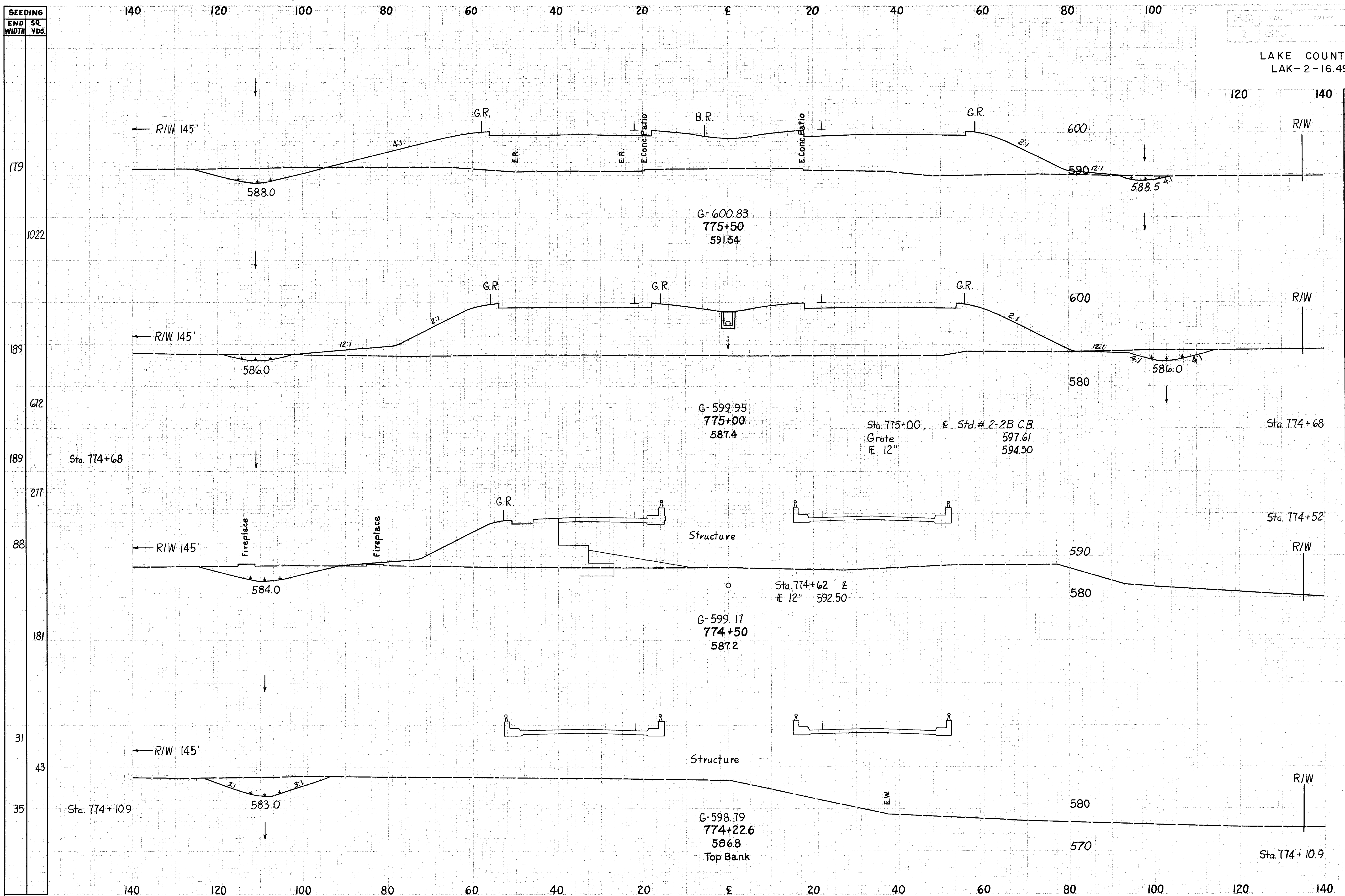
RELOCATION S.R.2 Sta. 774+22.6 to 775+50
