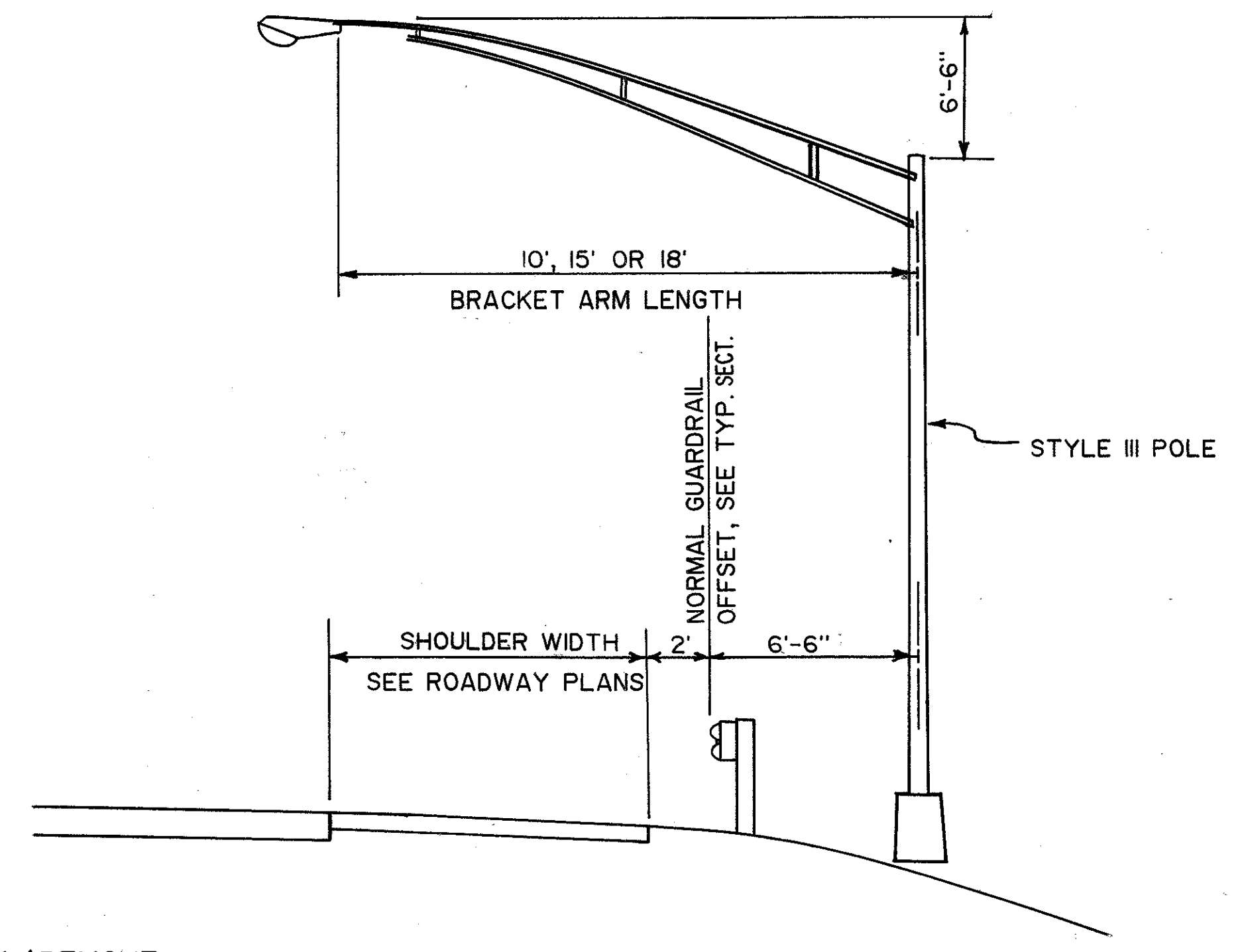
TYPICAL POLE PLACEMENT
