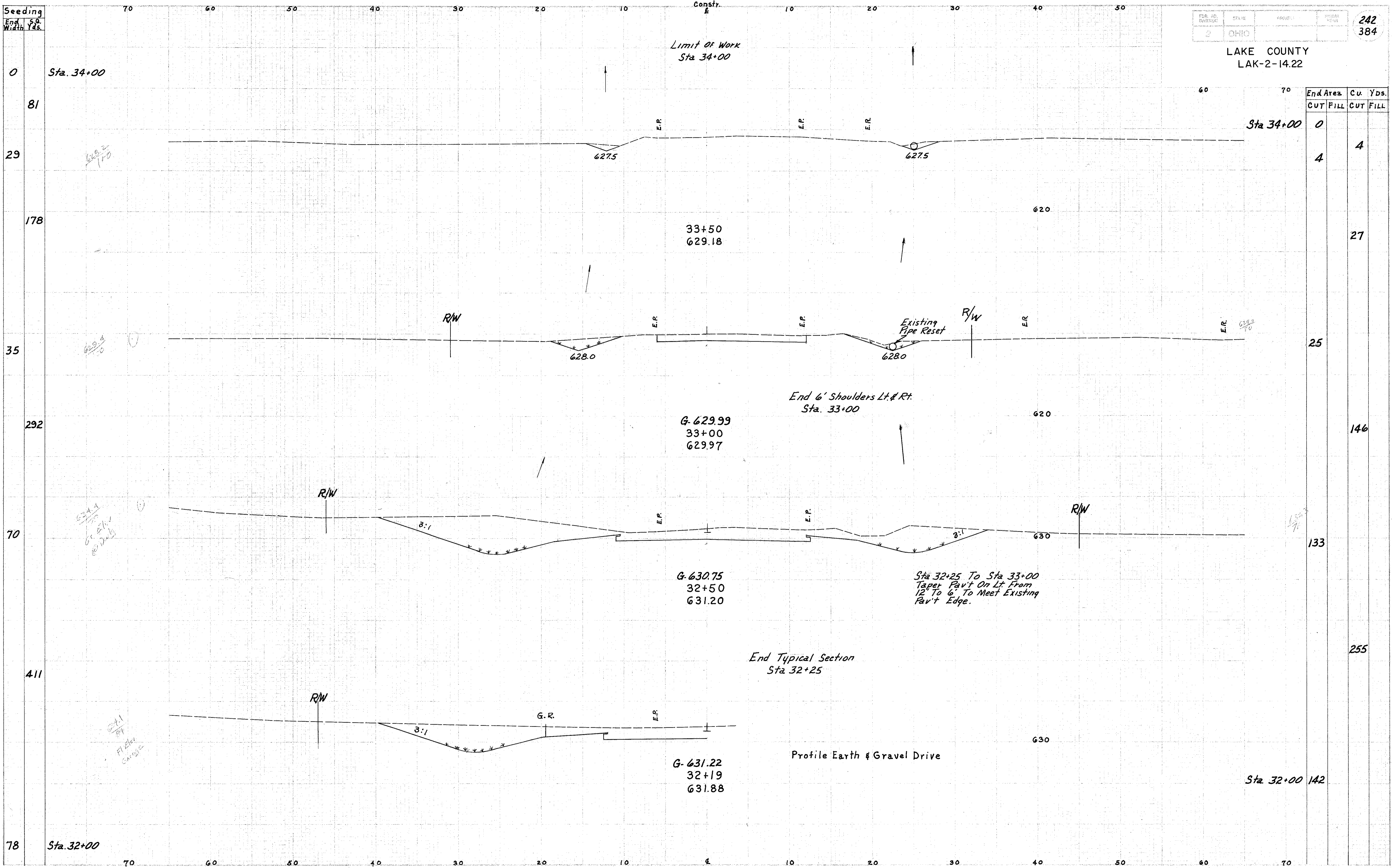
Reconstruction Elm Street Sta. 32+19 to 33+50
