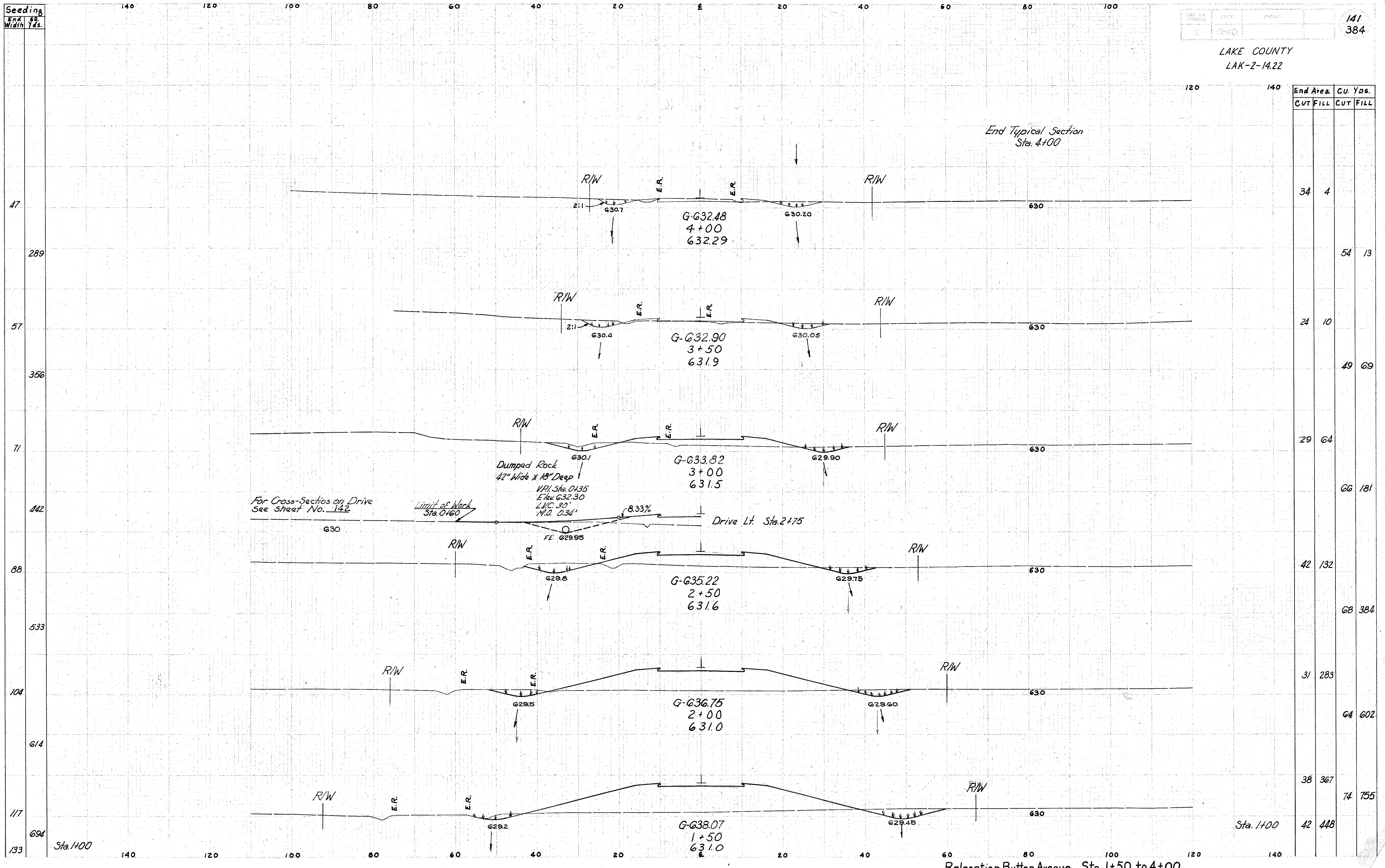
Relocation Button Avenue Sta. 1+50 to 4+00
